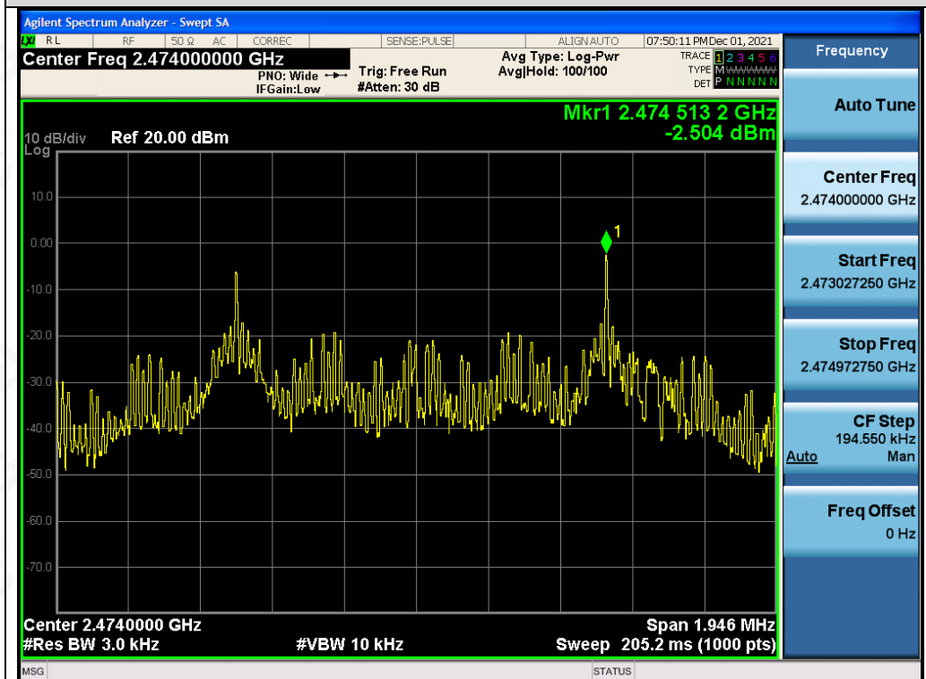
Test_Graph_FSK_ANT1_2474_2Mbps_PSD
