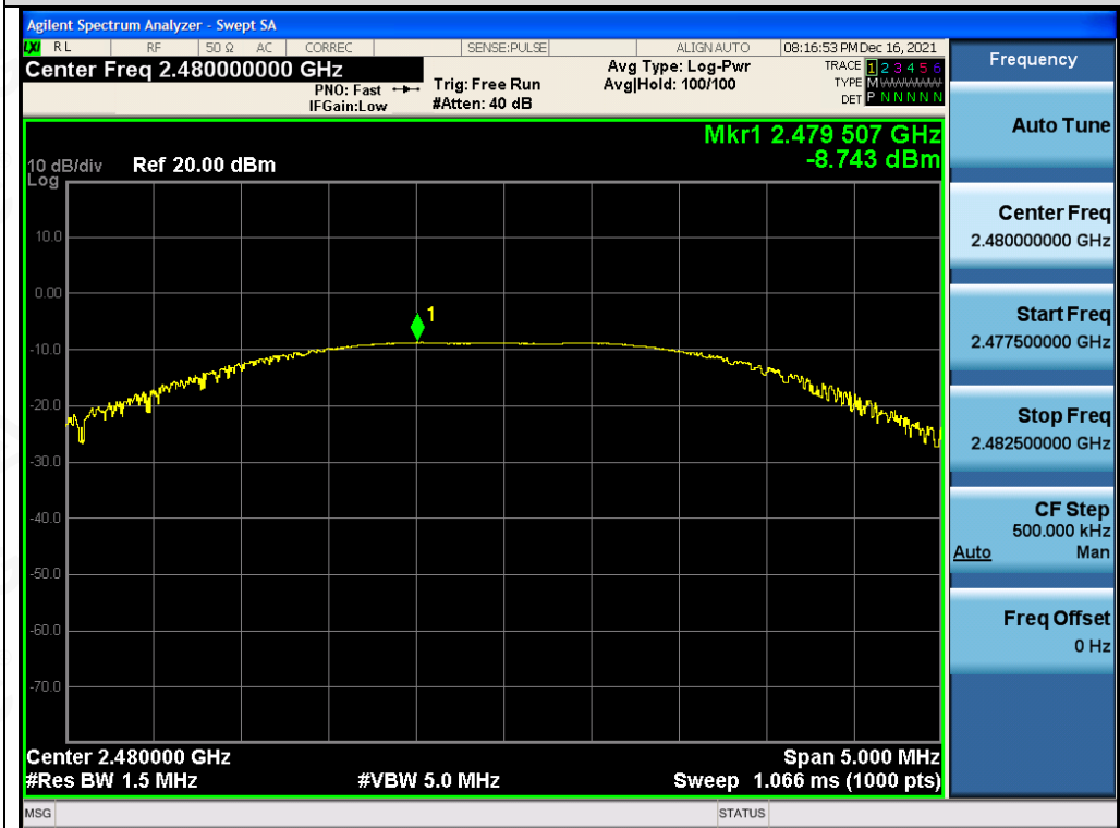
Test_Graph_FSK_ANT1_2480_2Mbps_Peak Power
