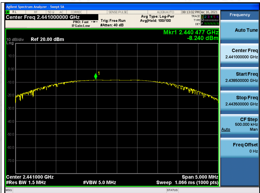
Test_Graph_FSK_ANT1_2441_2Mbps_Peak Power
