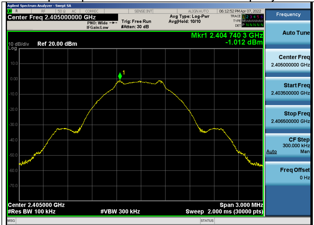
Test_Graph_GFSK_ANT1_2405_Reference Level
