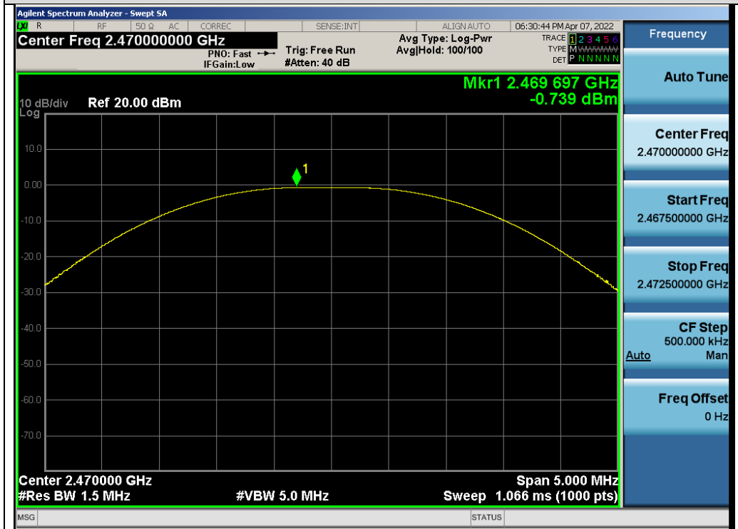
Test_Graph_GFSK_ANT1_2470_Peak Power
