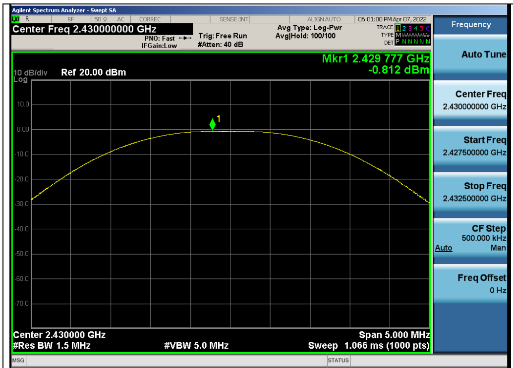
Test_Graph_GFSK_ANT1_2430_Peak Power
