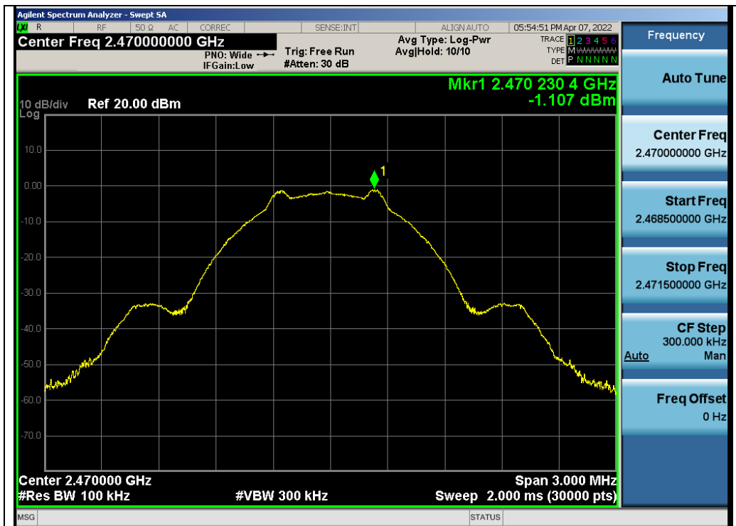
Test_Graph_GFSK_ANT1_2470_Reference Level
