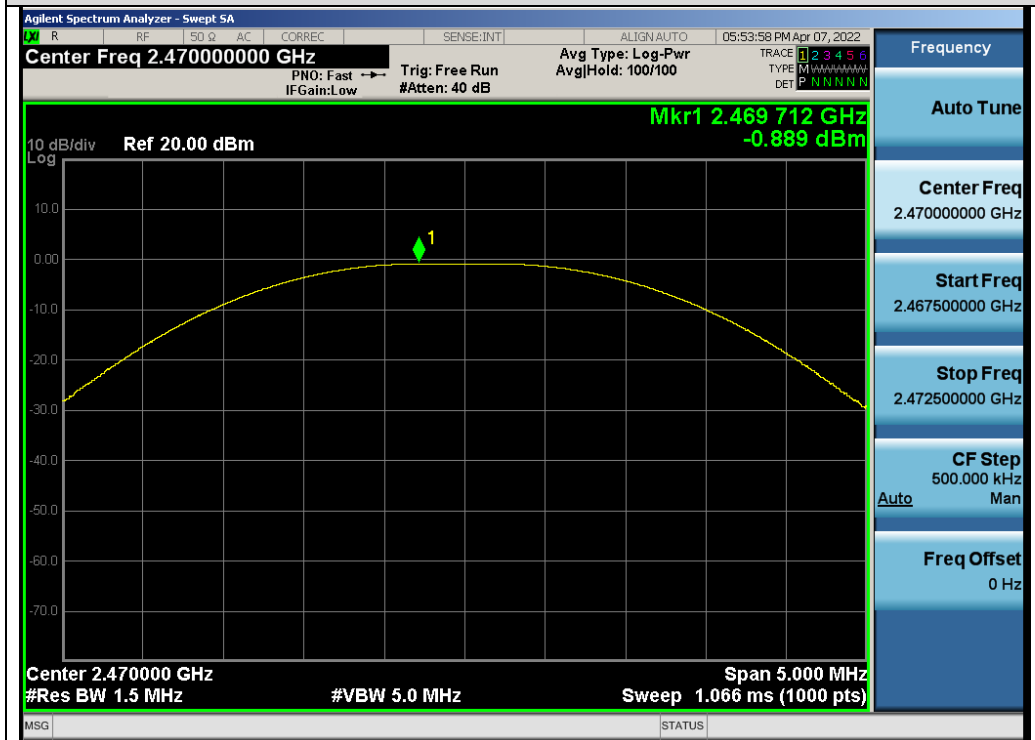
Test_Graph_GFSK_ANT1_2470_Peak Power
