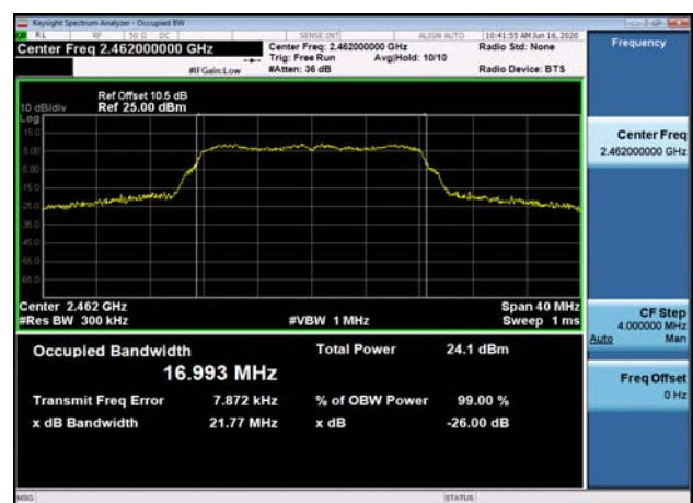
99% Bandwidth-802.11g,2462MHz
