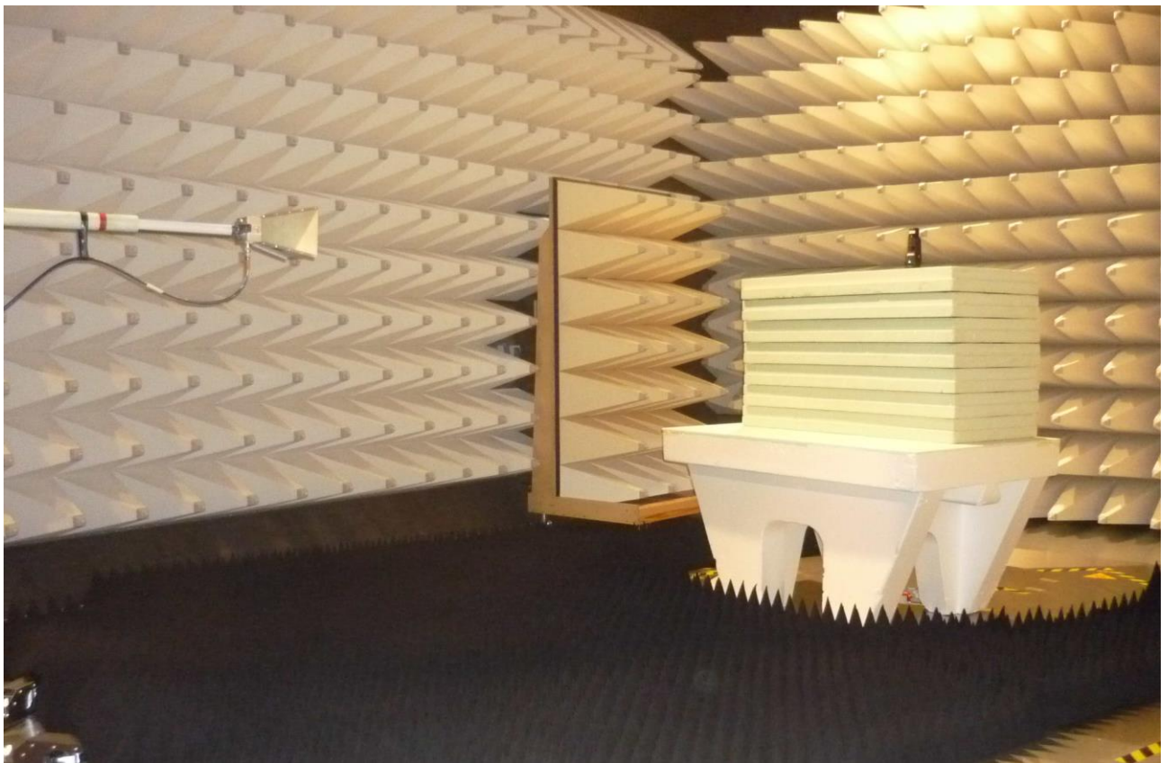
Tested frequency range > 1 GHz
