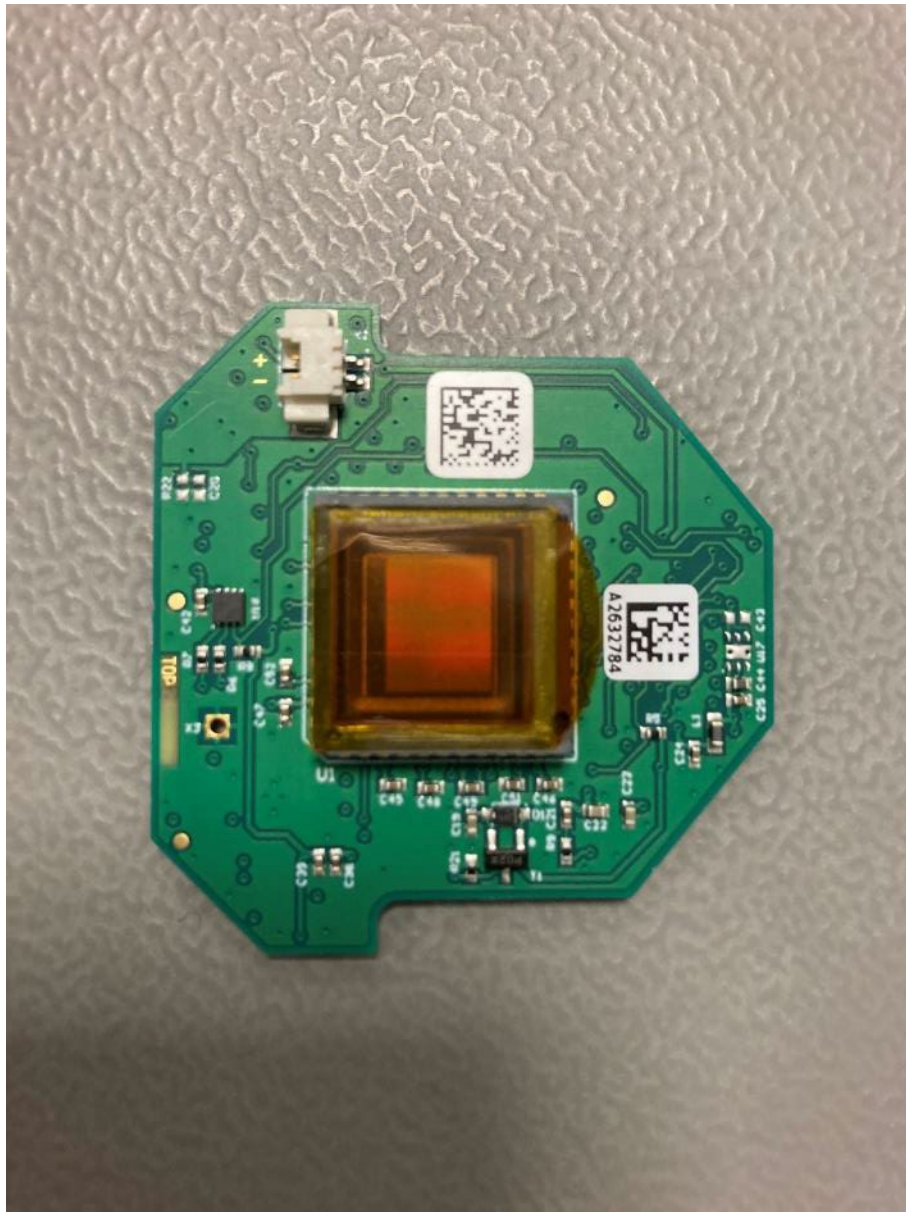
DFE Board (digital front end PCB) with infrared sensor
