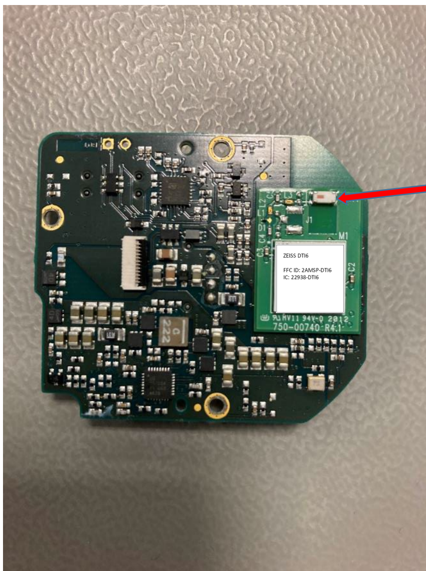
Charge PCB with Wifi board and ceramic chip antenna, top view
