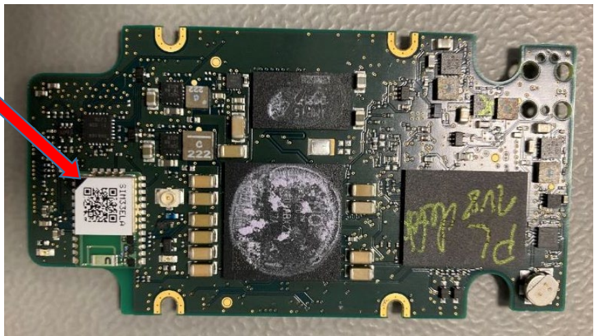
Mainboard PCB bottom without heat sink
