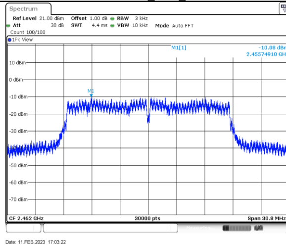
11N20SISO Ant1 2462
