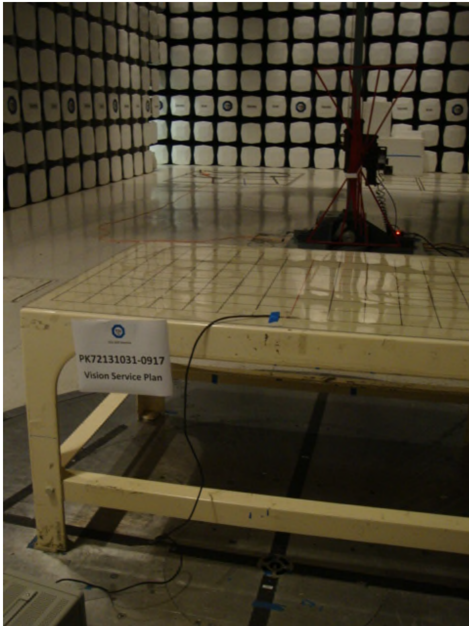
Radiated Emissions Test Setup (below 1GHz)
