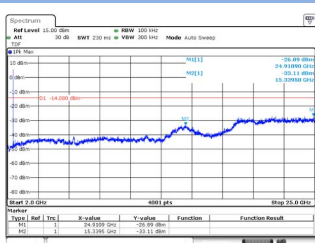
GFSK (BLE) LOW CHANNEL, SPURIOUS 2 GHz ~ 25 GHz
