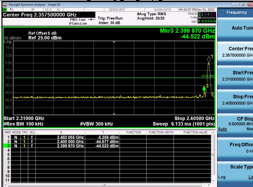
2 Bandedge_BLE_1Mbps_2402
