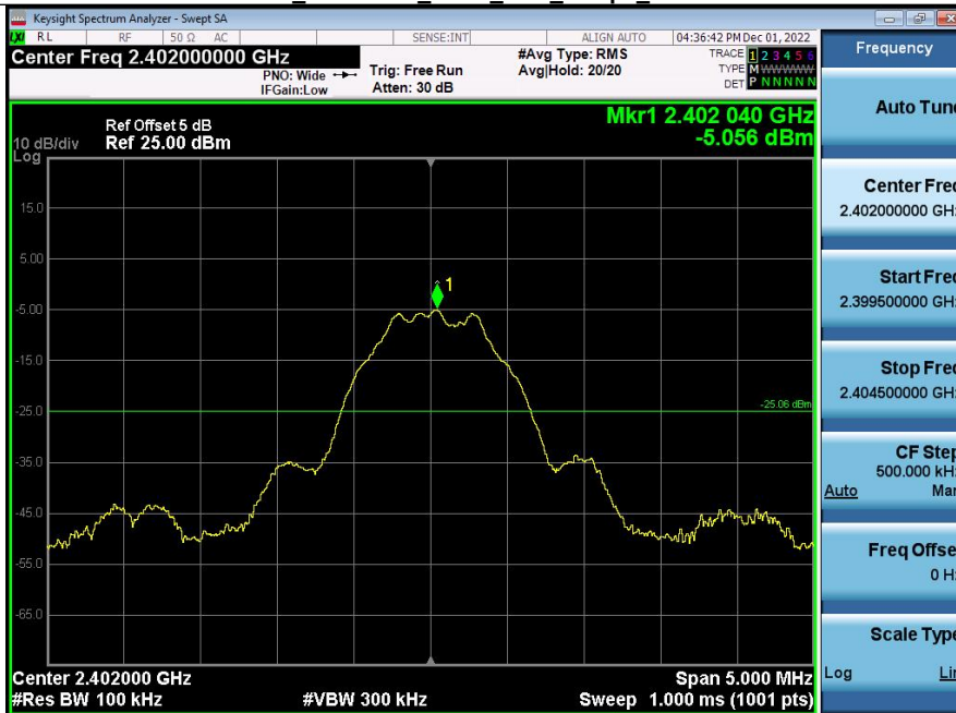
2 Bandedge_BLE_1Mbps_2402
