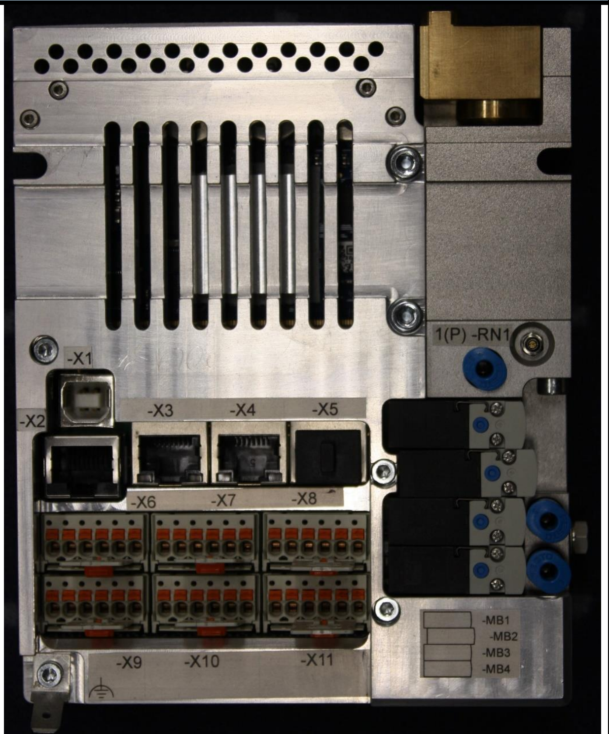
Backside view all markings will be engraved in series
