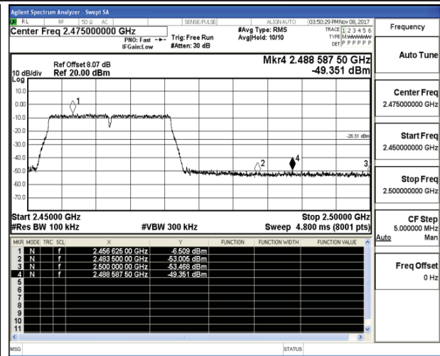
802.11n(HT20)-High channel
