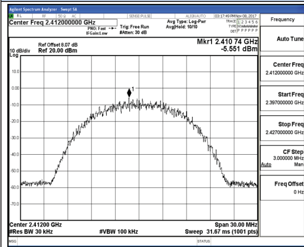
802.11b_Low Channel
