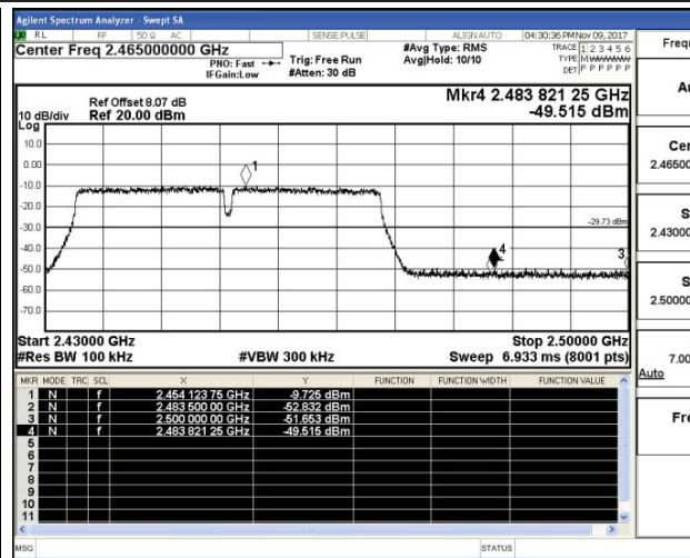
802.11n(HT40)-High channel
