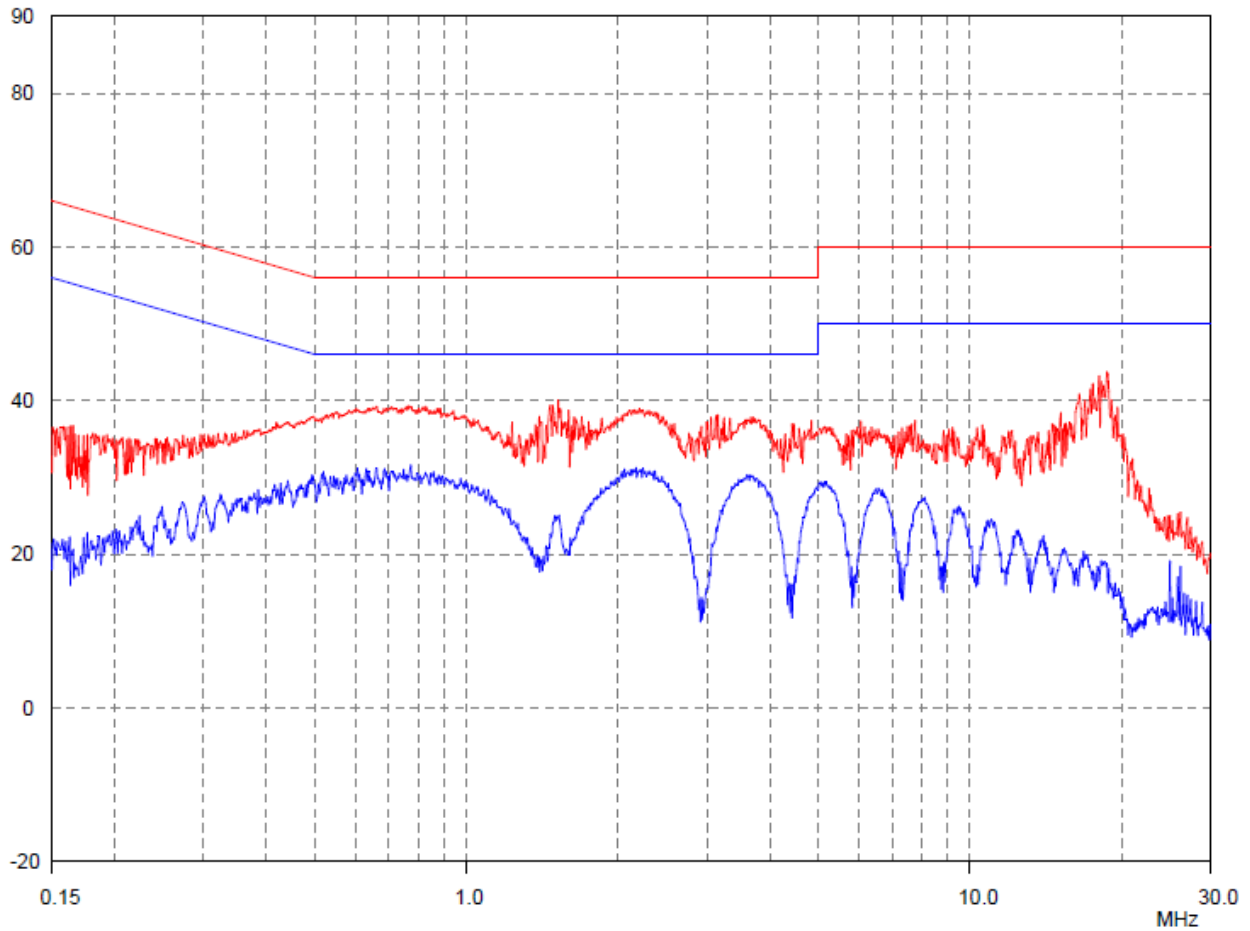
N Line
