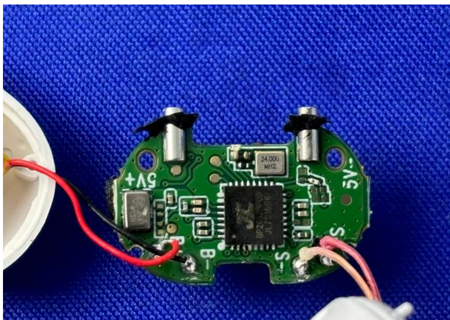
View of Product-3 L-ear
