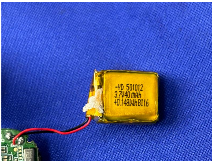
View of Product-6 L-ear
