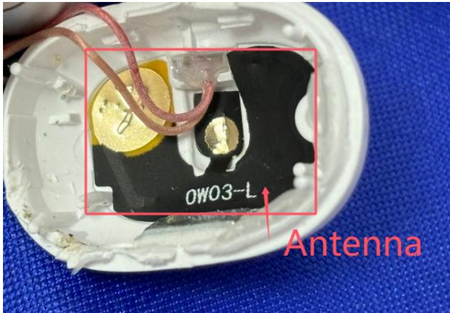
View of Product-5 L-ear
