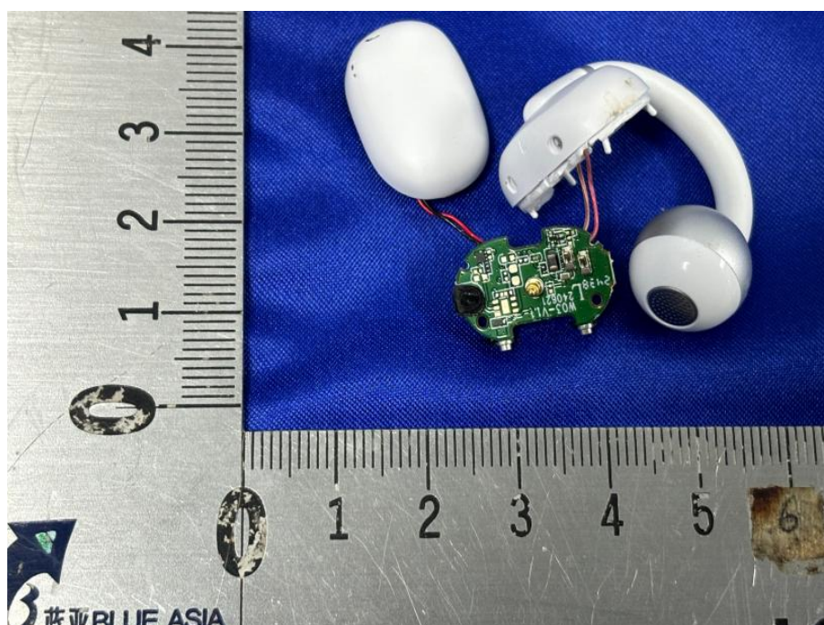
View of Product-2 L-ear
