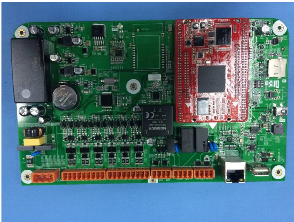
Mains Board PCB
