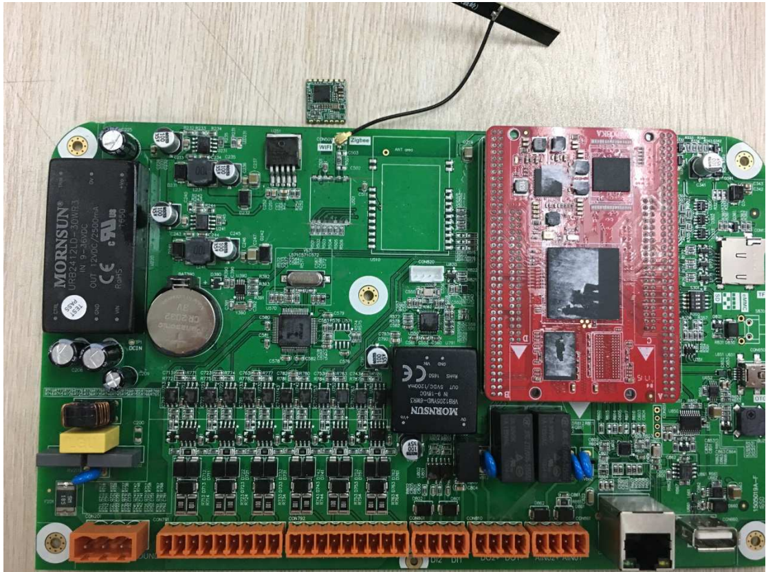
WiFi module view
