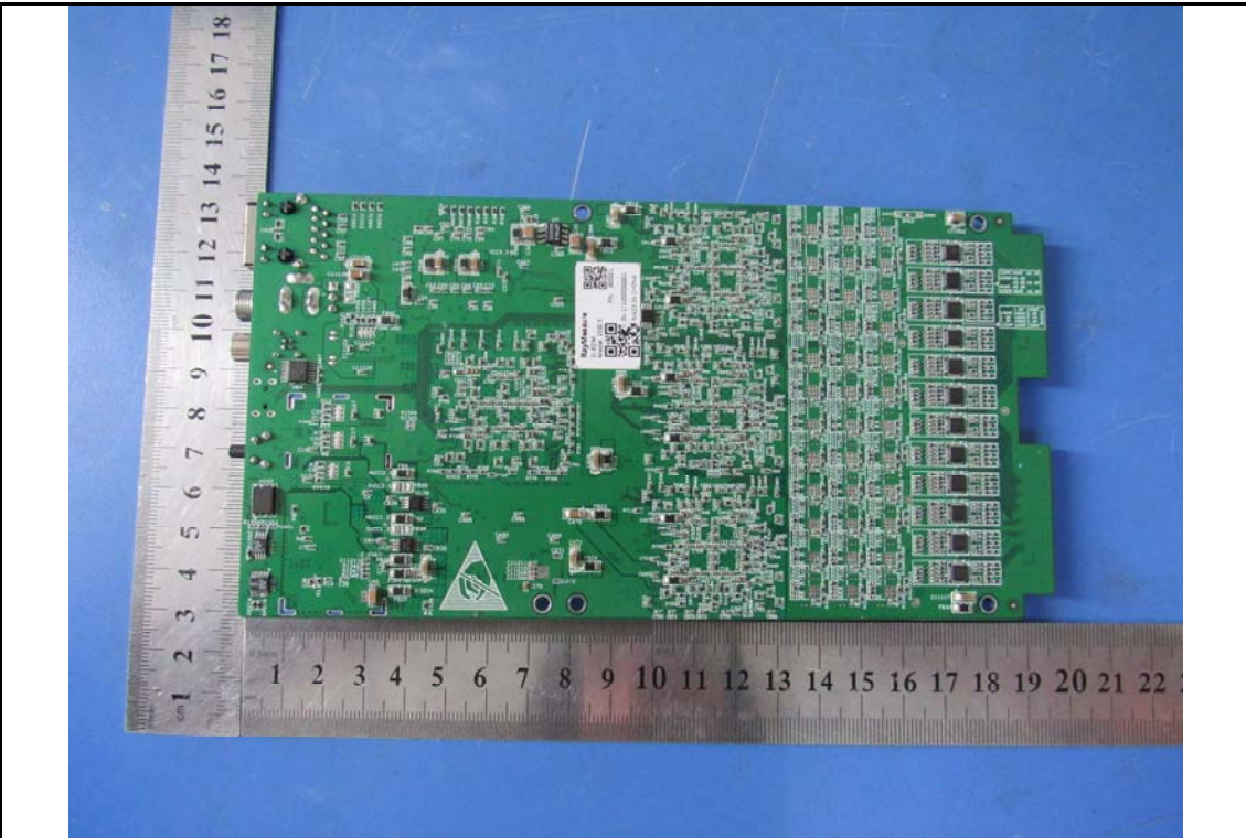
EUT PCBA – Rear View
