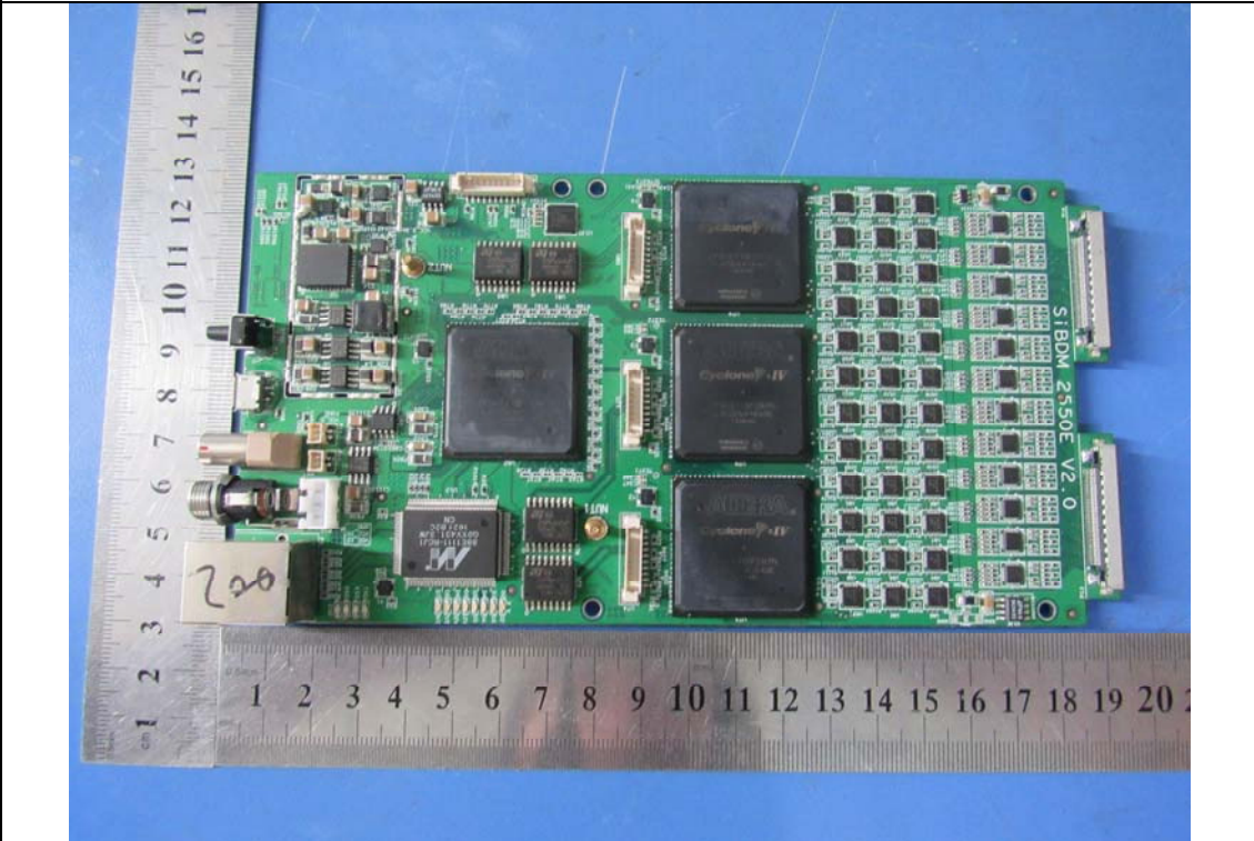
EUT PCBA Shielding Off – Front View
