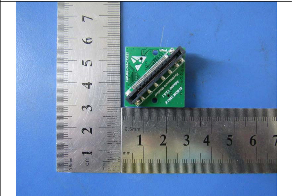
EUT Sensor PCBA 1 – Front View
