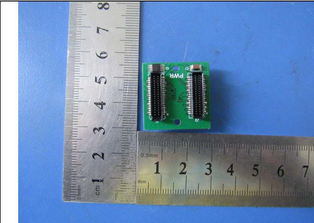
EUT Sensor PCBA 1 – Rear View
