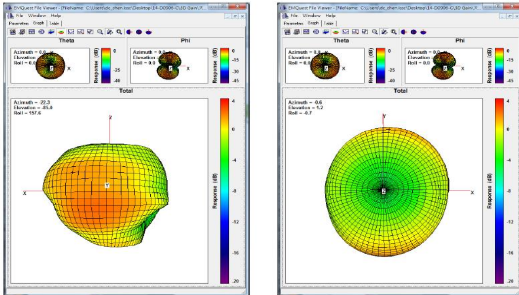
FIGURE 4-2: ANTENNA 3D RADIATION PATTERN @2441 MHz
