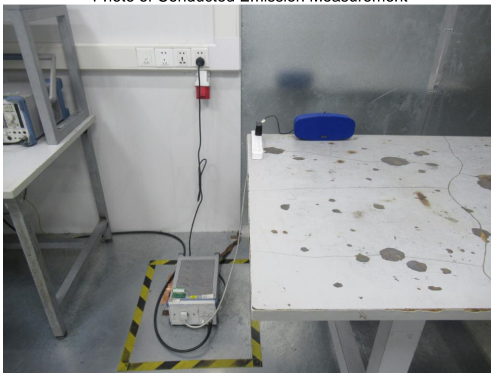
FCC ID: 2AMPLNAS-3105D Photo of Conducted Emission Measurement
