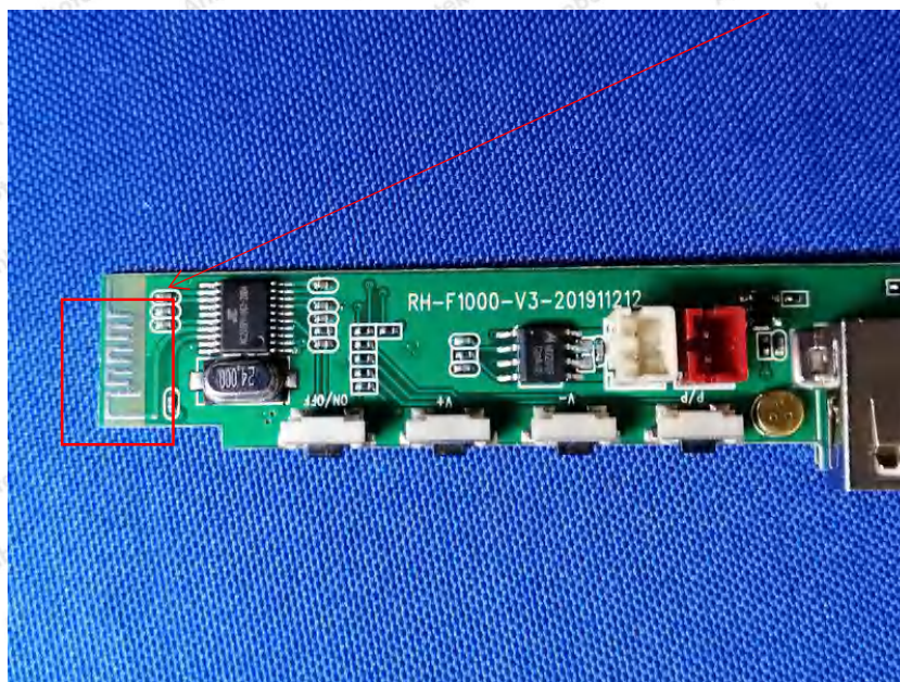
BT Antenna
