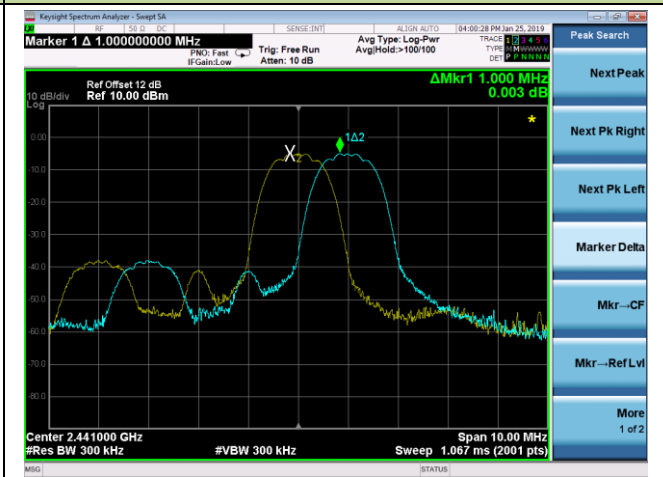
Channel 39 (2441MHz)
