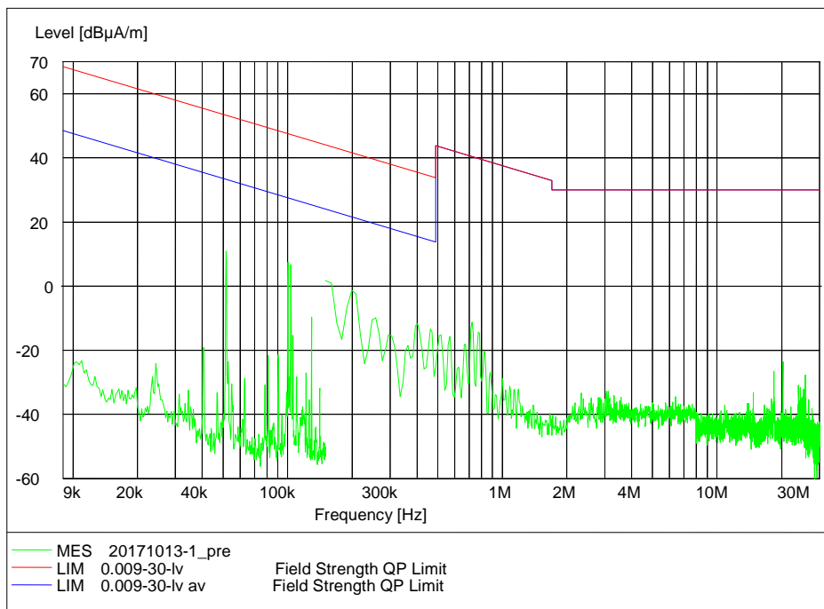
Frequency Range: 9Khz-30MHz Detector: QP mode Modulation type: GFSK (LE)
