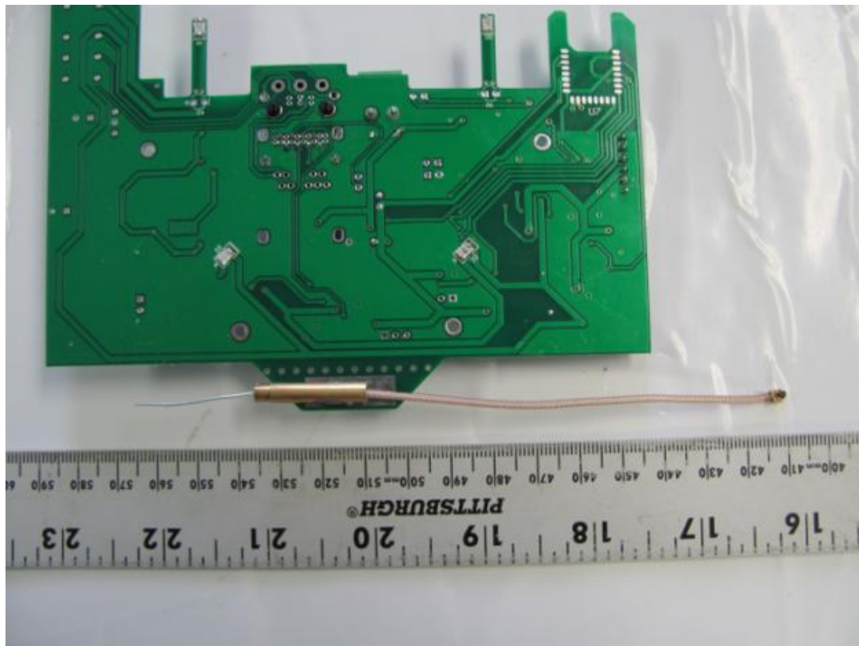
Figure 4. 2.4 GHz ISM Radio Module Antenna
