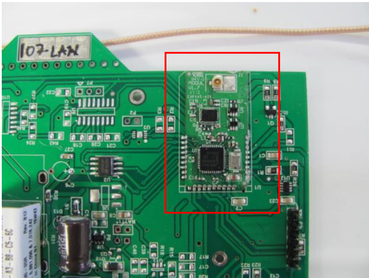
Figure 2. 2.4 GHz ISM Radio Module
