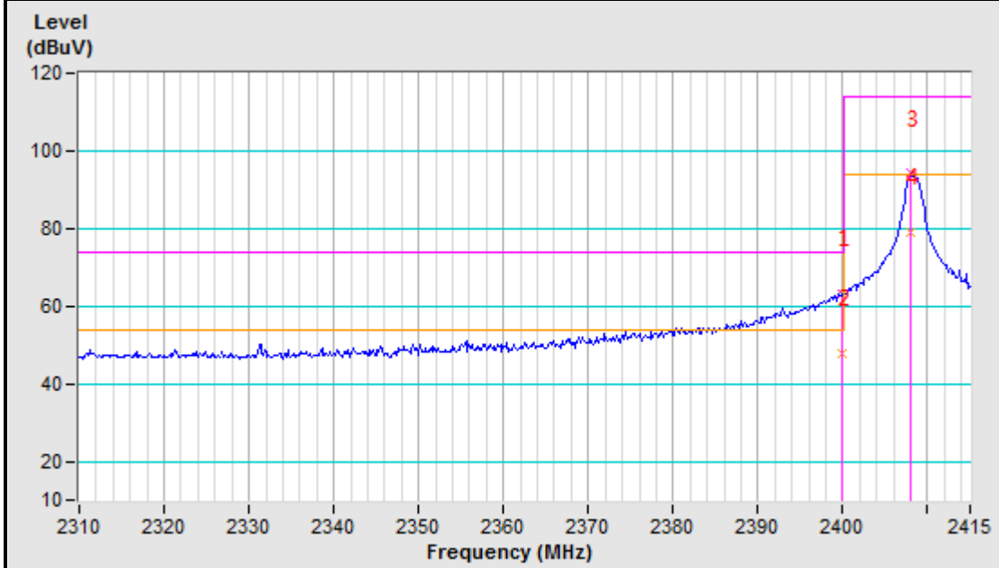
2408MHz Vertical
