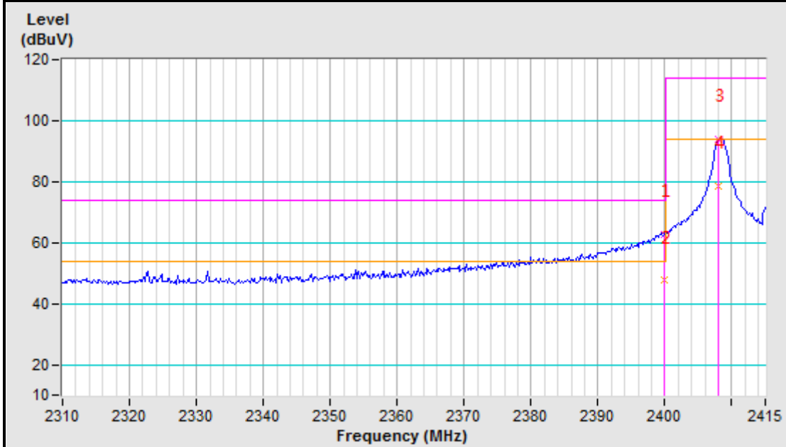
2408MHz Vertical
