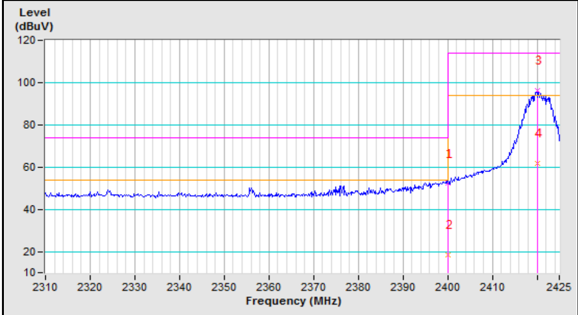
2420MHz Vertical
