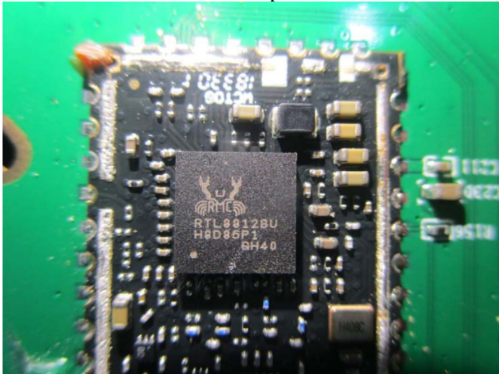
RF Chip
