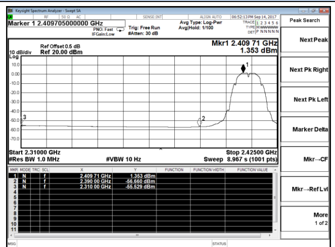
Channel 1 / 2412 MHz – Average
