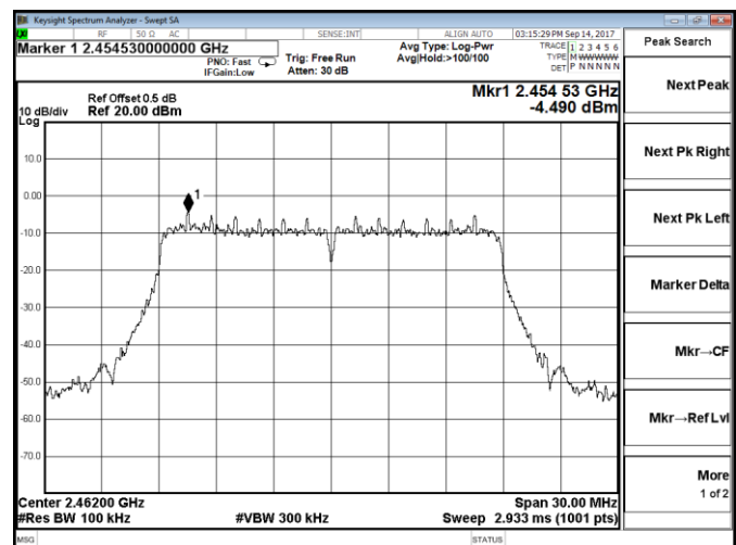
802.11n-HT20 Chain 1-High channel
