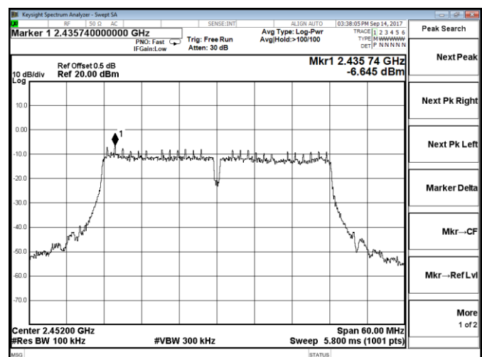
802.11n-HT40 Chain 1-High channel
