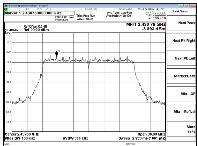
802.11n-HT20 Chain 1-Middle channel
