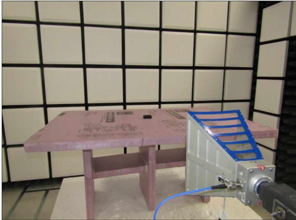
Figure 3: Radiated Emissions – 960MHz to 18GHz – Front View
