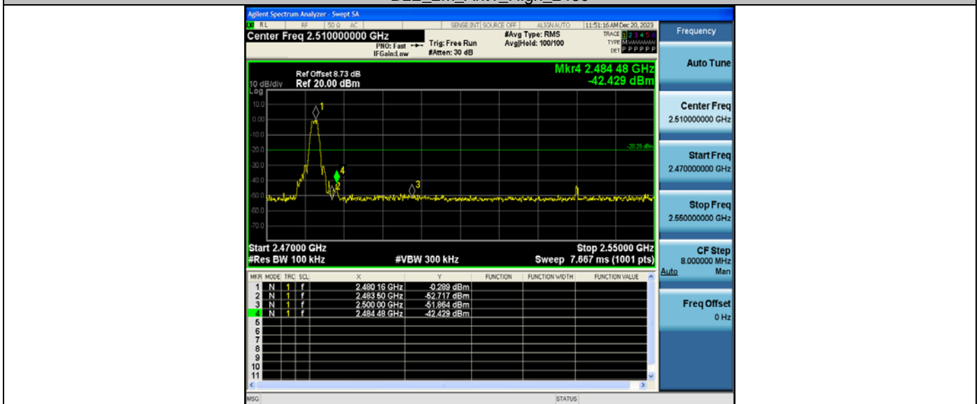
BLE_2M_Ant1_High_2480
