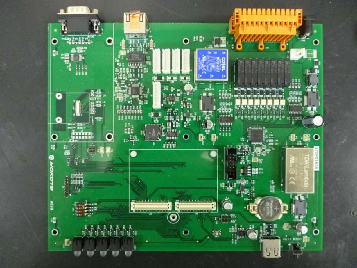
CPU Board
