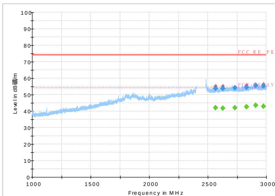
Fig 46. Radiated Spurious Emission (802.11b,Ch11,1GHz~3GHz)
