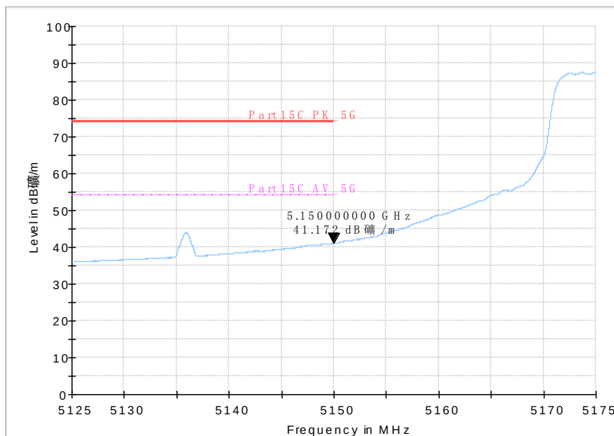
Fig. 56 Band Edges (802.11n-HT20, 5180MHz)
