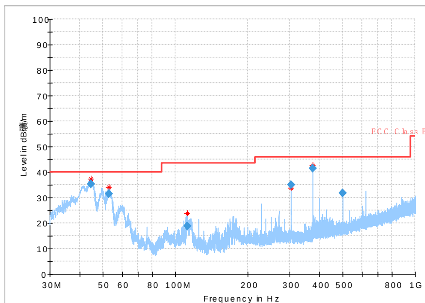
Fig. 80 Radiated Spurious Emission (802.11ac-HT20, Ch36, 30 MHz-1 GHz)
