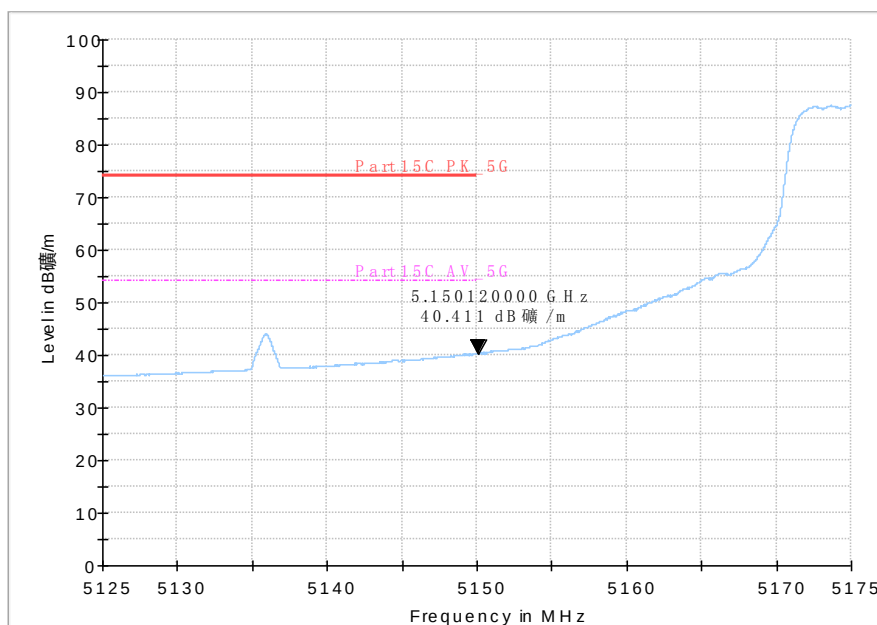
Fig. 58 Band Edges (802.11n-HT40, 5190MHz)
