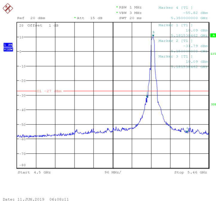
Fig. 43 Band Edges (802.11a, 5180MHz)
