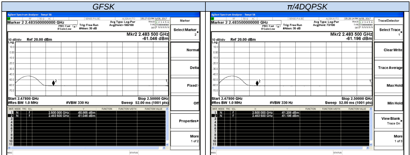
Channel 78 / 2480 MHz – Non-Hopping – Average
