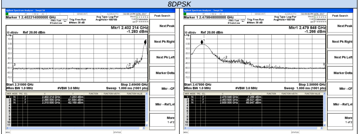
Channel 0 / 2402 MHz – Non-Hopping – Peak
