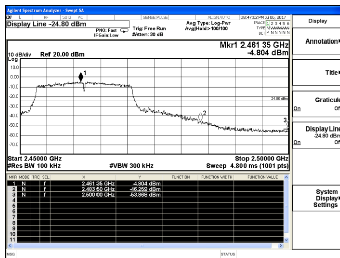
802.11n-HT20-High channel
