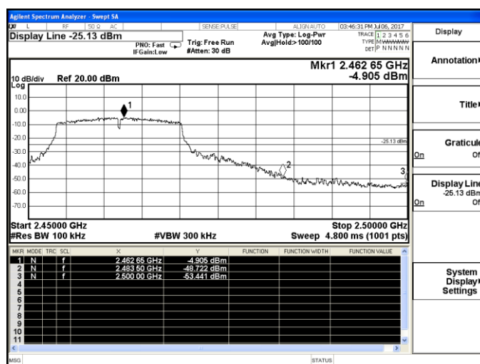
802.11g-High channel
