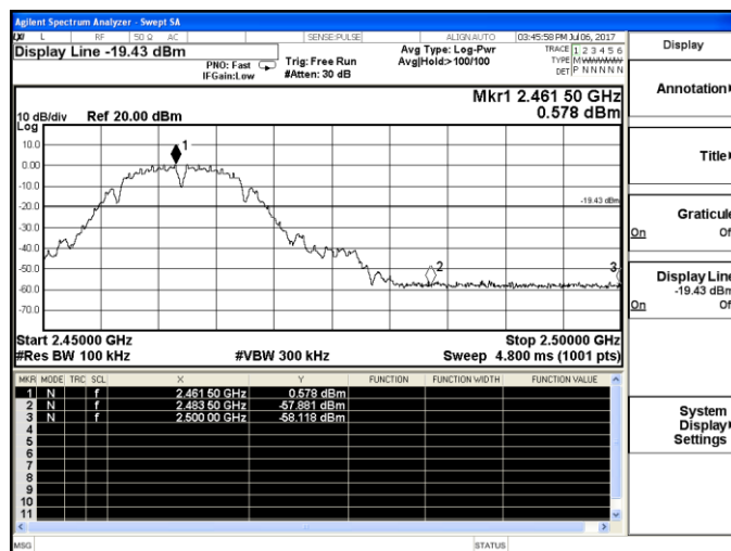
802.11b-High channel
