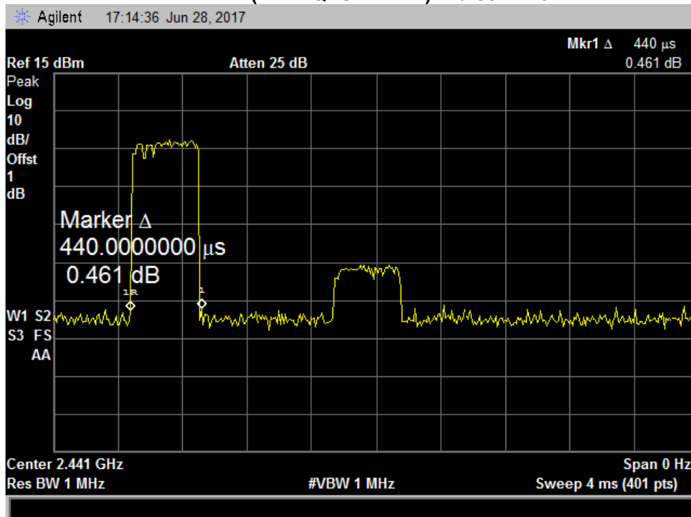
2441 MHz ( \pi/4 -DQPSK 2DH1)- Pulse Time
