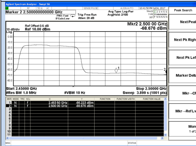
Channel 1 / 2462 MHz – Average
