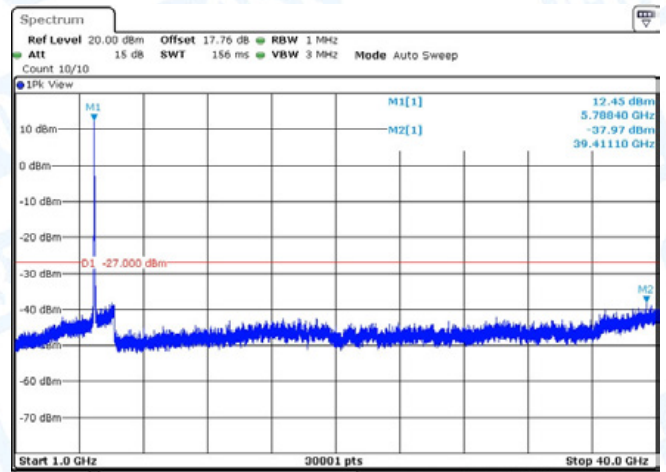
11N40-CDD-Ant1-5795-1000~40000-PASS
