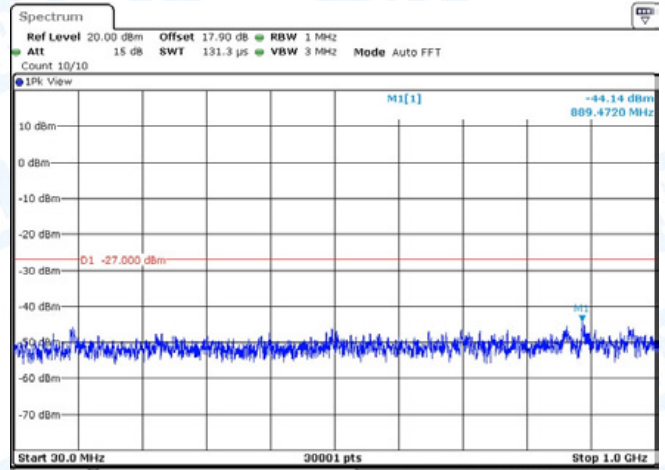
11AC20-CDD-Ant1-5720-30~1000-PASS
