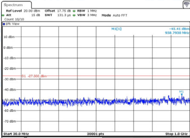
11N40-CDD-Ant2-5755-30~1000-PASS
