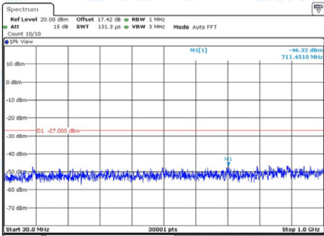
11N40-CDD-Ant2-5230-30~1000-PASS
