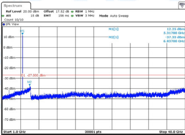
11AC20-CDD-Ant1-5320-1000~40000-PASS
