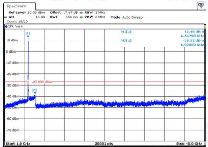
11N40-CDD-Ant1-5550-1000~40000-PASS
