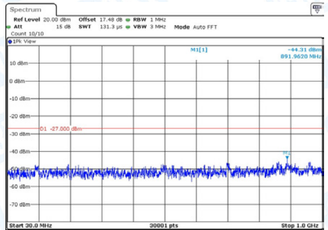
11AC20-CDD-Ant1-5200-30~1000-PASS
