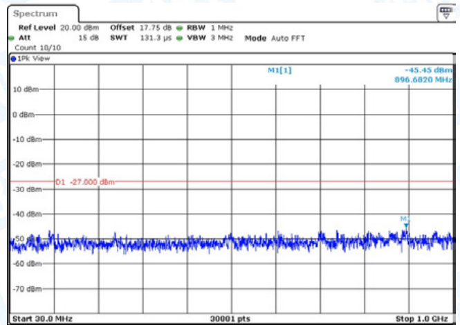
11AC20-CDD-Ant2-5720-30~1000-PASS
