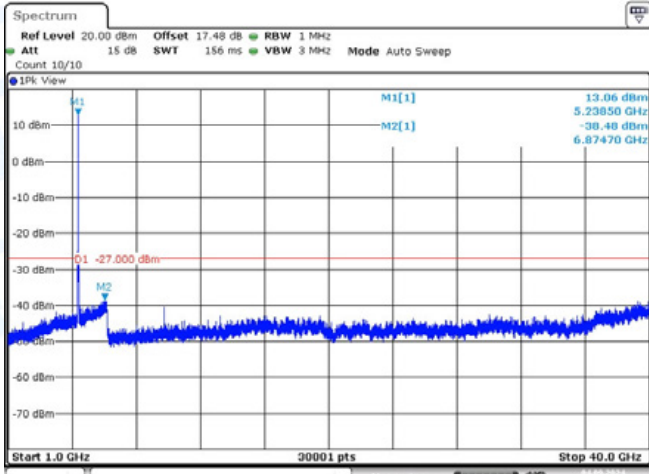
11AC20-CDD-Ant2-5200-1000~40000-PASS
