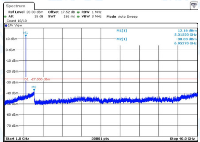
11N20-CDD-Ant1-5320-1000~40000-PASS
