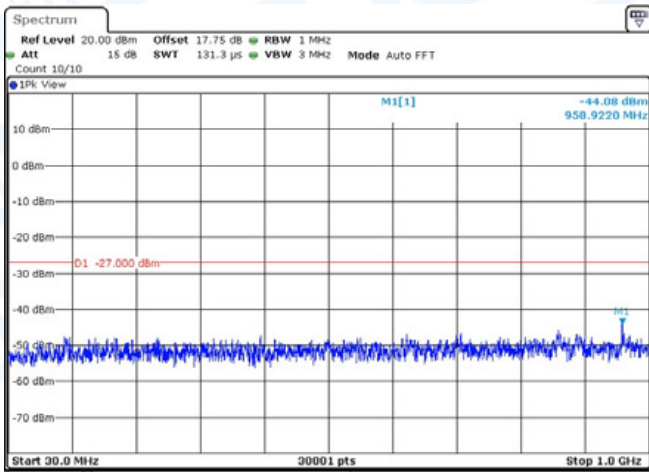
11N40-CDD-Ant2-5710-30~1000-PASS
