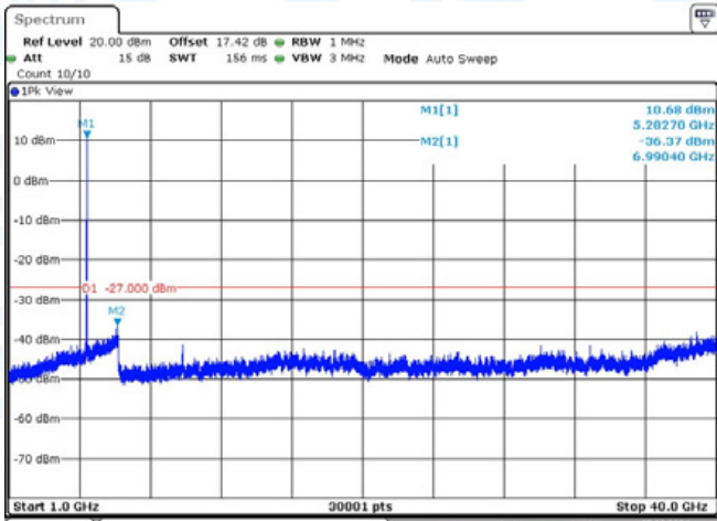
11AC20-CDD-Ant2-5260-1000~40000-PASS
