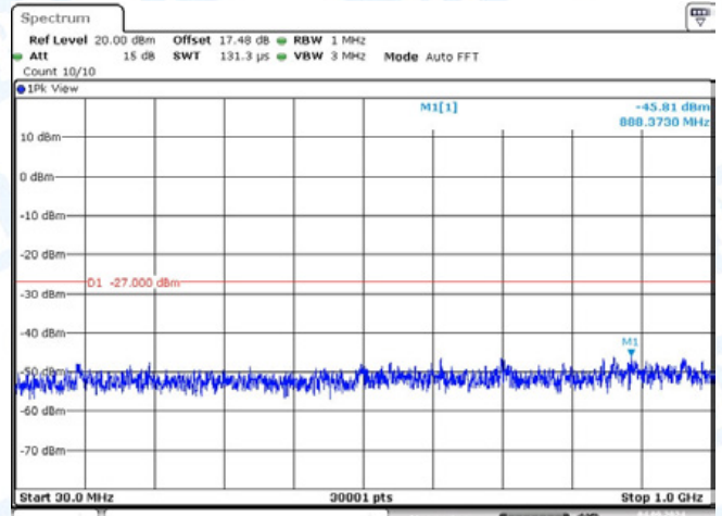
11AC20-CDD-Ant1-5240-30~1000-PASS
