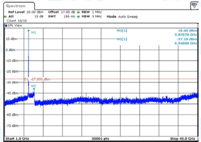
11N20-CDD-Ant1-5825-1000~40000-PASS
