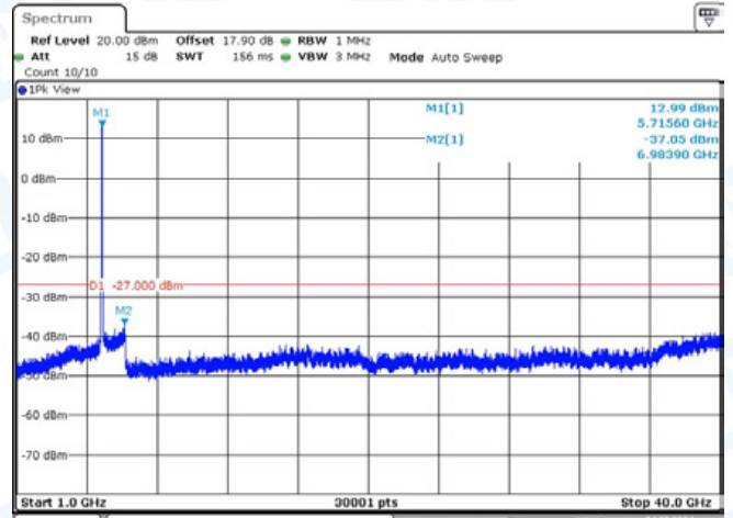
11N40-CDD-Ant1-5710-1000~40000-PASS
