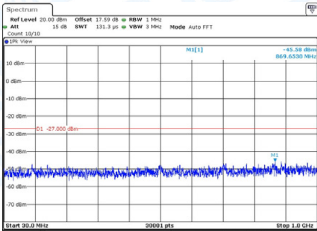
11N20-CDD-Ant2-5500-30~1000-PASS
