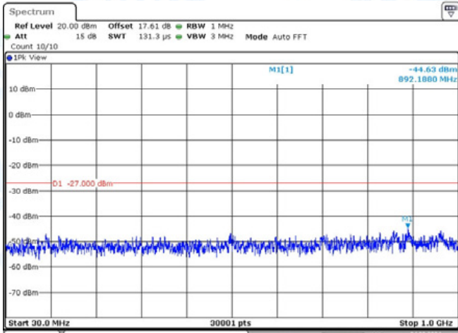
11N40-CDD-Ant2-5510-30~1000-PASS
