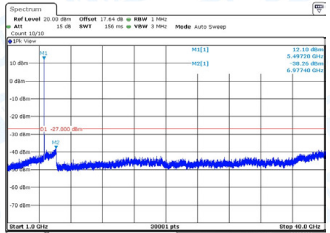
11N20-CDD-Ant1-5500-1000~40000-PASS
