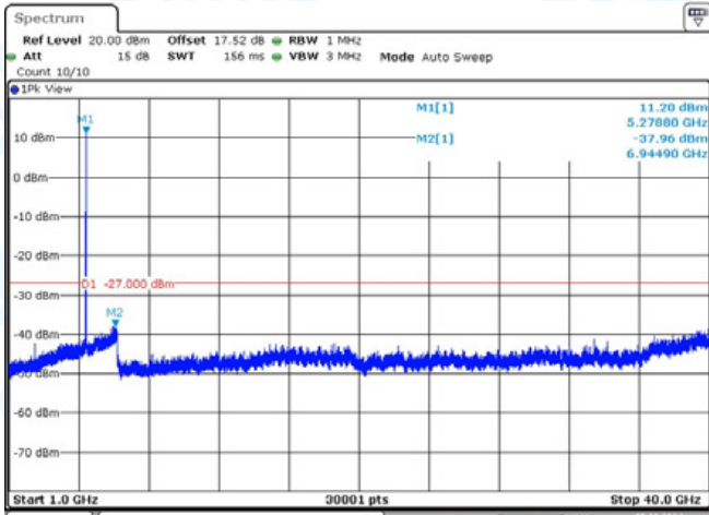
11AC20-CDD-Ant2-5280-1000~40000-PASS
