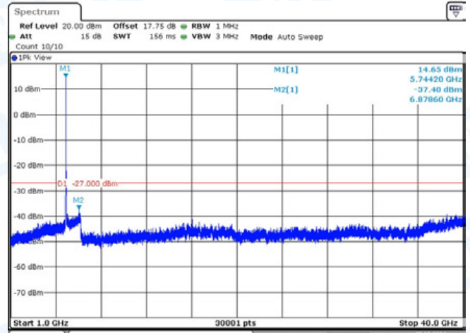
11N20-CDD-Ant1-5745-1000~40000-PASS
