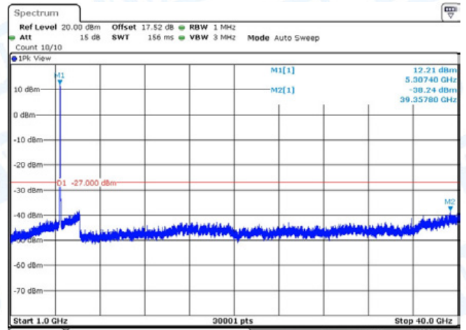
11N40-CDD-Ant1-5310-1000~40000-PASS
