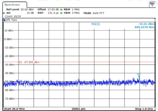
11AC20-CDD-Ant1-5580-30~1000-PASS
