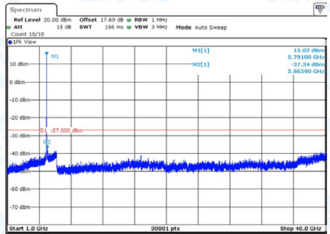
11N20-CDD-Ant2-5745-1000~40000-PASS
