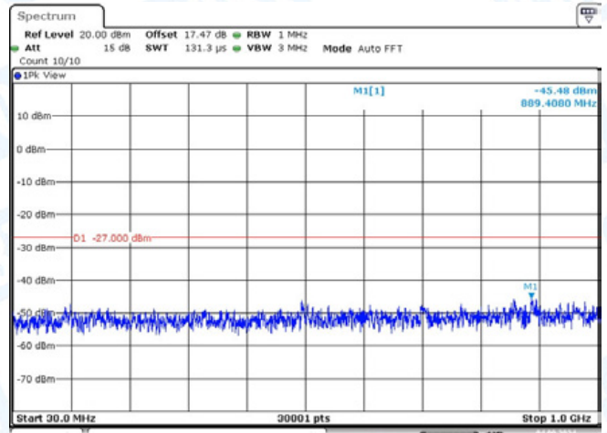
11AC20-CDD-Ant2-5240-30~1000-PASS
