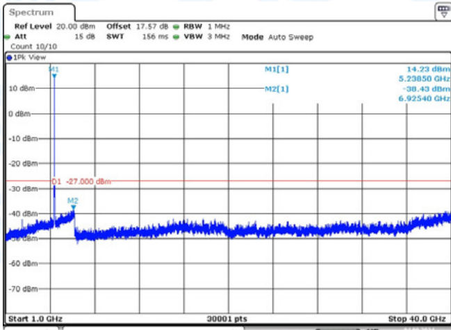
11AC20-CDD-Ant1-5240-1000~40000-PASS
