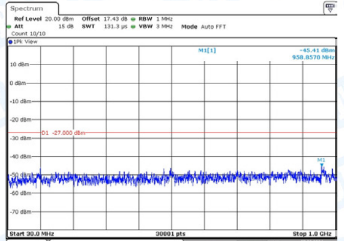
11AC20-CDD-Ant1-5320-30~1000-PASS
