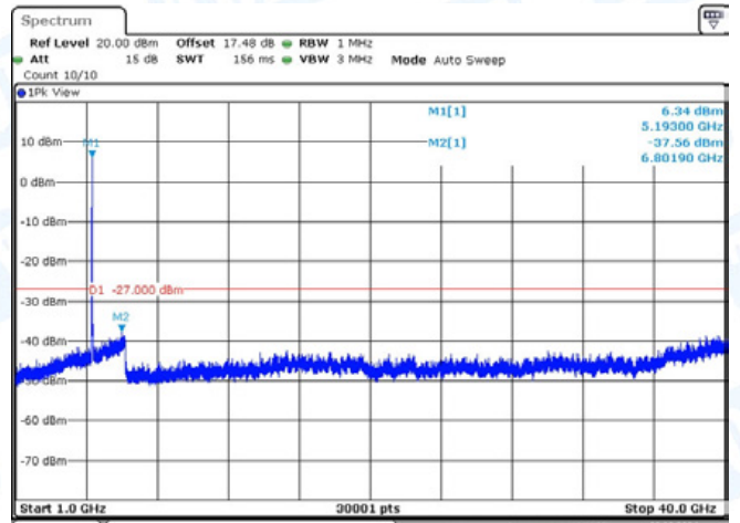
11N40-CDD-Ant1-5190-1000~40000-PASS
