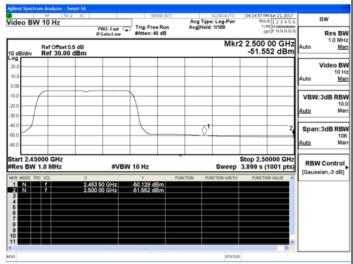
802.11g-High channel(Average)
