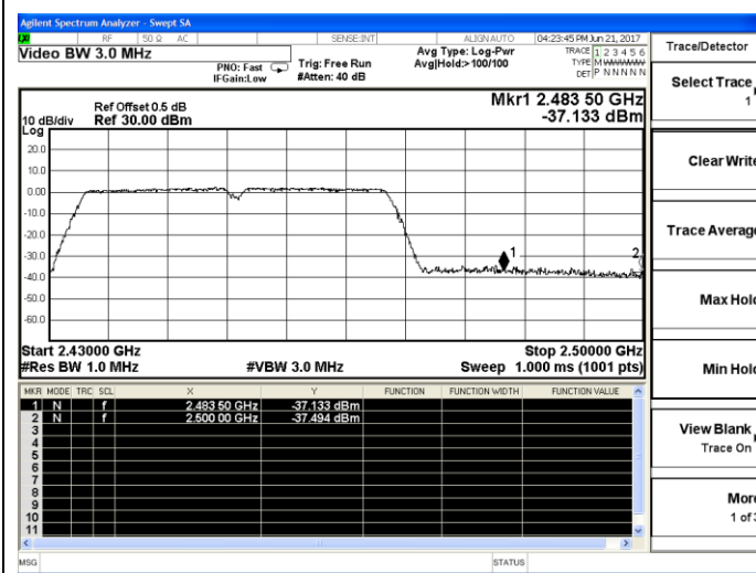
802.11n-HT40-High channel(Peak)
