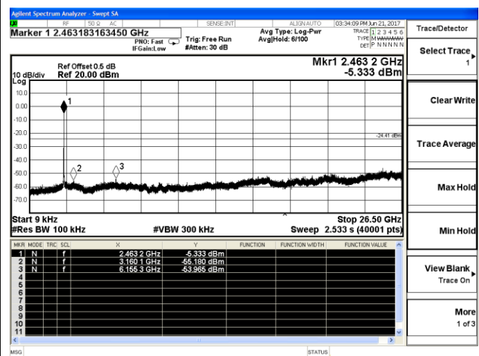
802.11n-HT20-High channel
