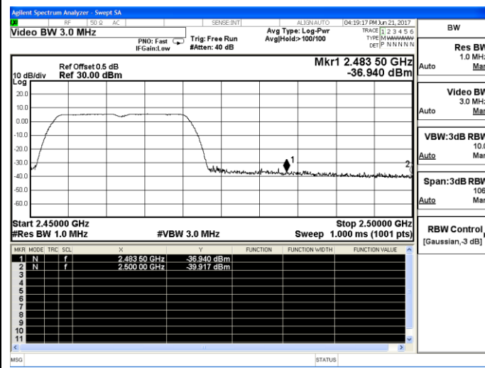
802.11n-HT20-High channel(Peak)
