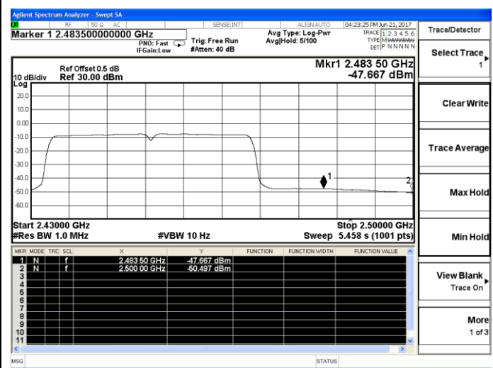
802.11n-HT40-High channel(Average)
