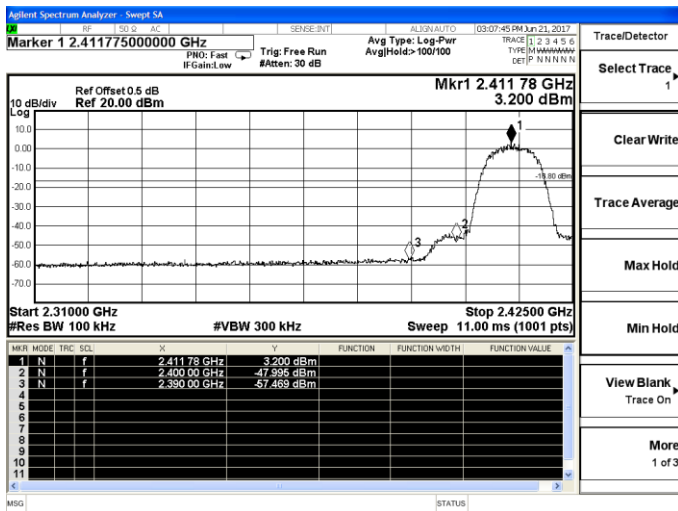
802.11b-Low channel
