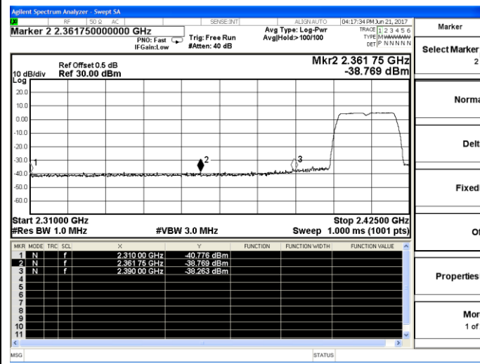
802.11n-HT20-Low channel(Peak)
