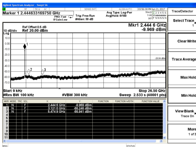
802.11n-HT40-Middle channel
