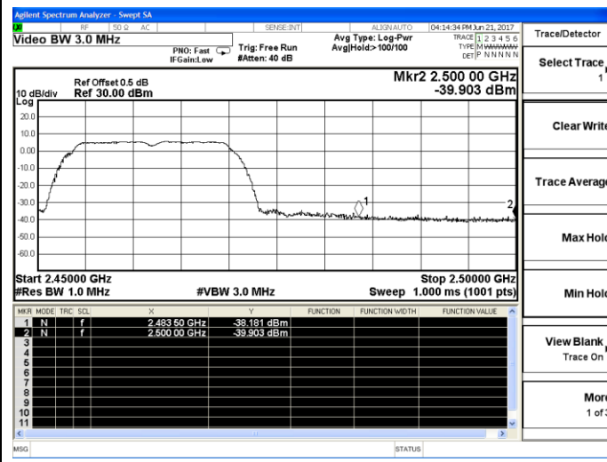
802.11g-High channel(Peak)
