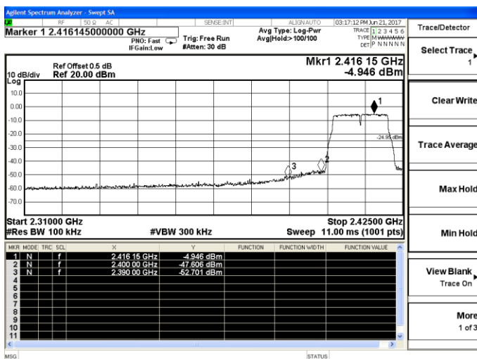
802.11g-Low channel
