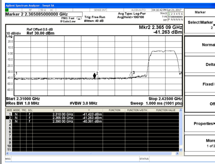
802.11g-Low channel(Peak)
