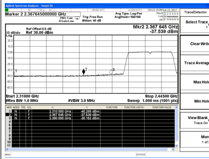
802.11n-HT40-Low channel(Peak)
