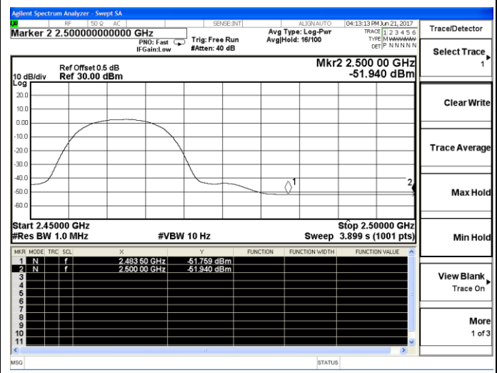
802.11b-High channel(Average)
