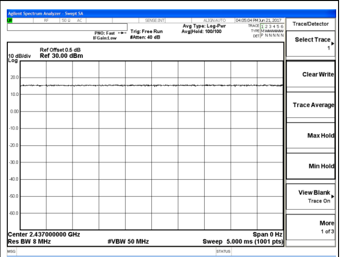
802.11g
