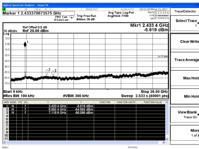
802.11g-Middle channel
