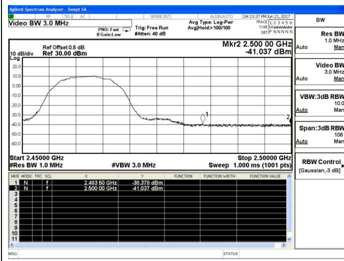
802.11b-High channel(Peak)
