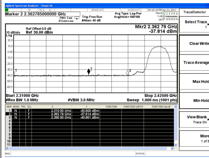
802.11b-Low channel(Peak)
