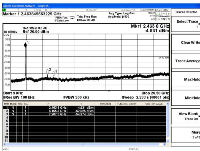
802.11g-High channel
