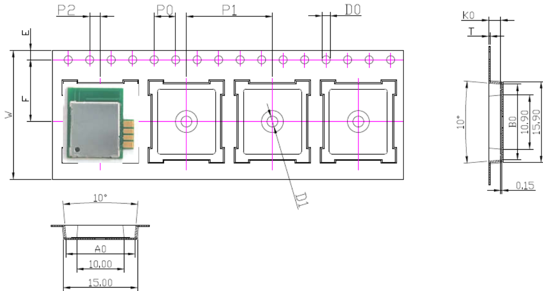
FIG 8 Carrier size
