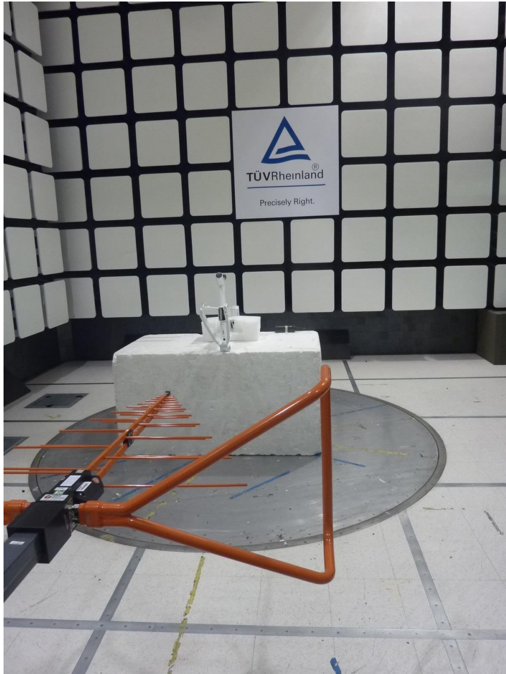
Figure 2: Test Setup for Radiated Emissions 30 MHz to 1000 MHz
