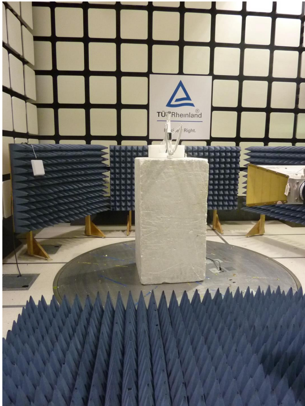
Figure 3: Test Setup for Radiated Emissions 1 GHz to 18 GHz
