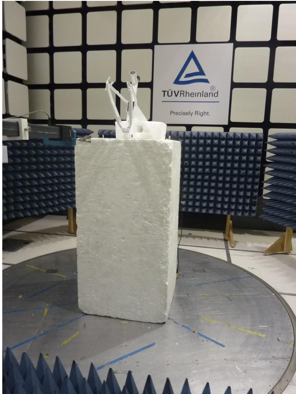
Figure 4: Test Setup for Radiated Emissions 18 GHz to 25 GHz
