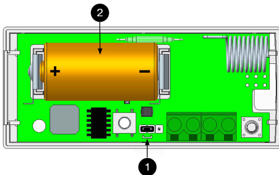
Figure 3.8: Install battery
