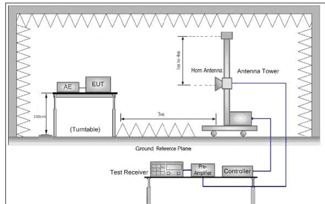
Figure 3. Above 1 GHz
