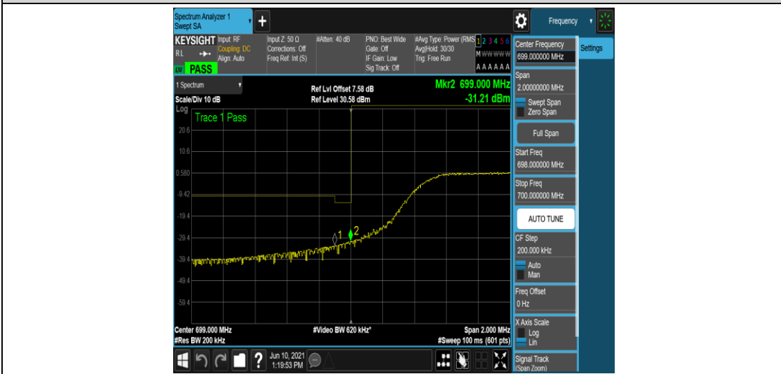
Band12-10MHz-QPSK-23130-1RB#0
