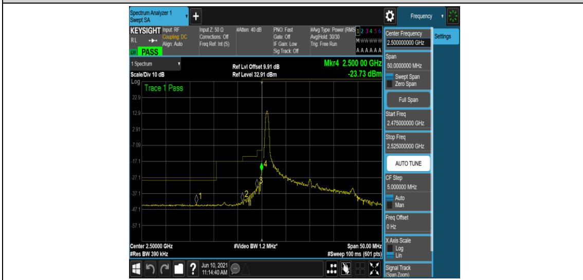
Band7-20MHz-QPSK-20850-1RB#99
