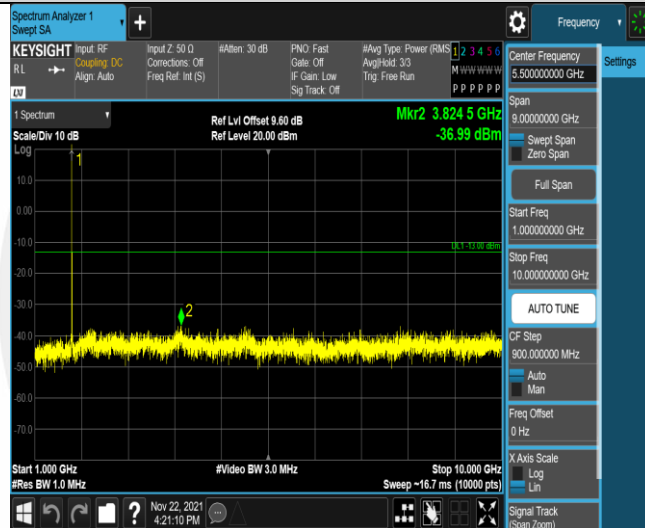
Band66-5MHz-QPSK-131997-1RB#0-Range2:1000~10000MHz
