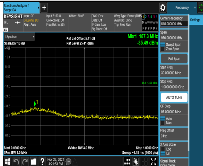
Band66-5MHz-QPSK-132322-1RB#0-Range1:30~1000MHz
