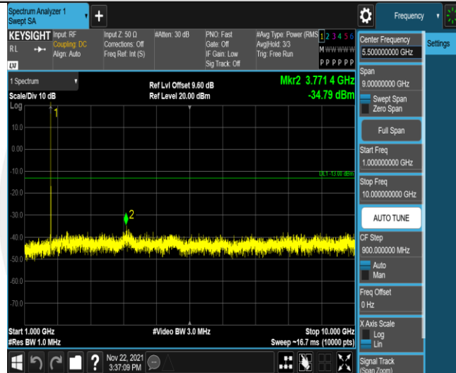
Band66-3MHz-16QAM-131987-1RB#0-Range2:1000~10000MHz
