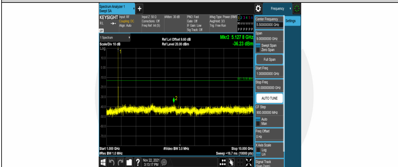
Band66-1.4MHz-16QAM-131979-1RB#0-Range2:1000~10000MHz
