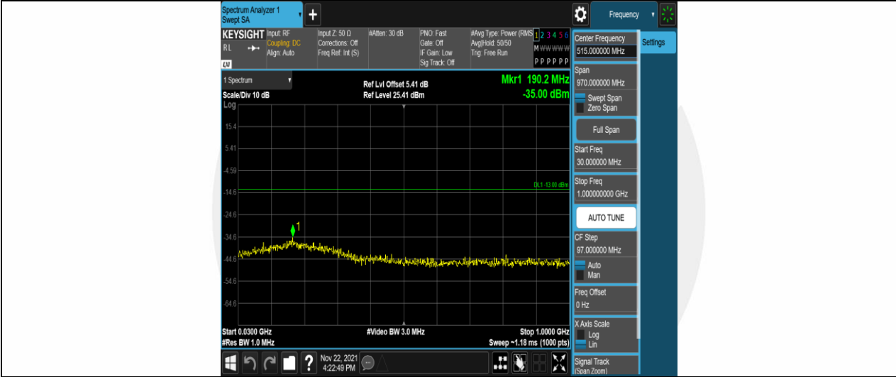
Band66-5MHz-QPSK-132647-1RB#0-Range1:30~1000MHz
