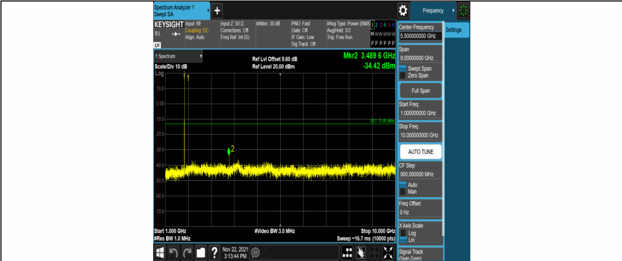
Band66-1.4MHz-QPSK-132322-1RB#0-Range2:1000~10000MHz
