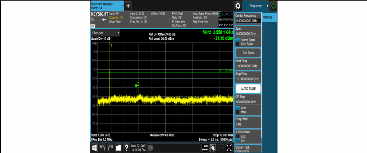
Band66-1.4MHz-QPSK-132665-1RB#0-Range2:1000~10000MHz
