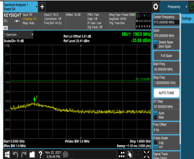
Band66-3MHz-16QAM-132657-1RB#0-Range1:30~1000MHz
