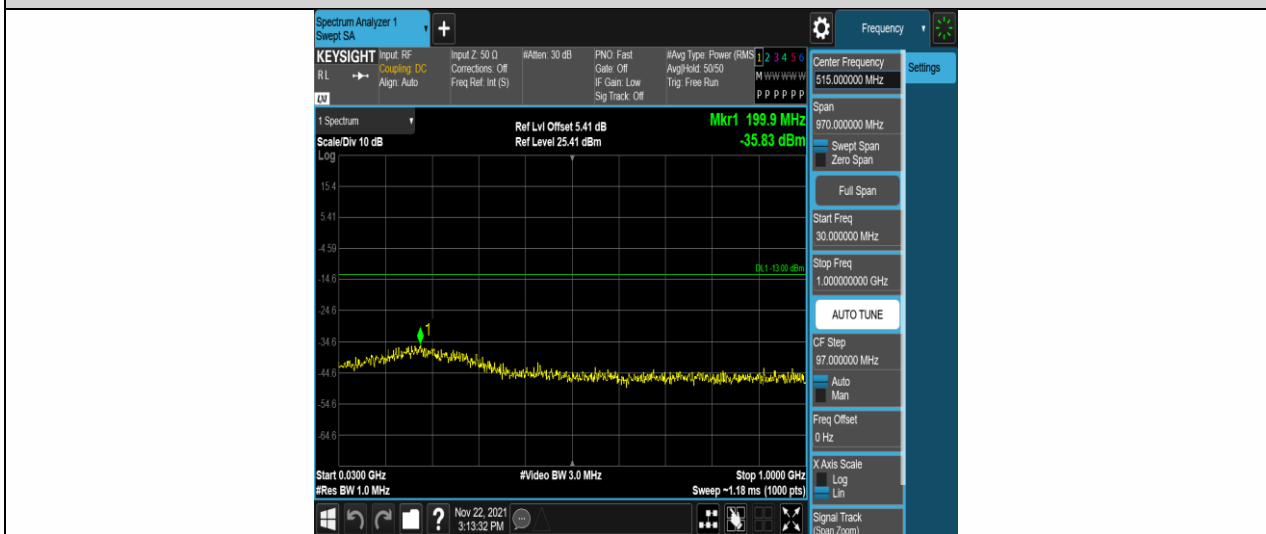
Band66-1.4MHz-QPSK-132322-1RB#0-Range1:30~1000MHz
