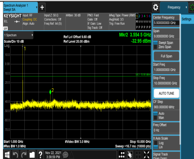
Band66-3MHz-16QAM-132657-1RB#0-Range2:1000~10000MHz
