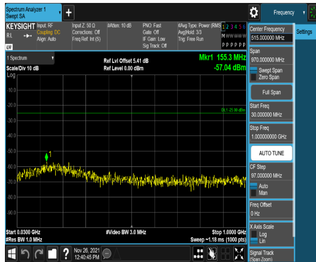
Band7-20MHz-16QAM-20850-100RB#0-Range1:30~1000MHz
