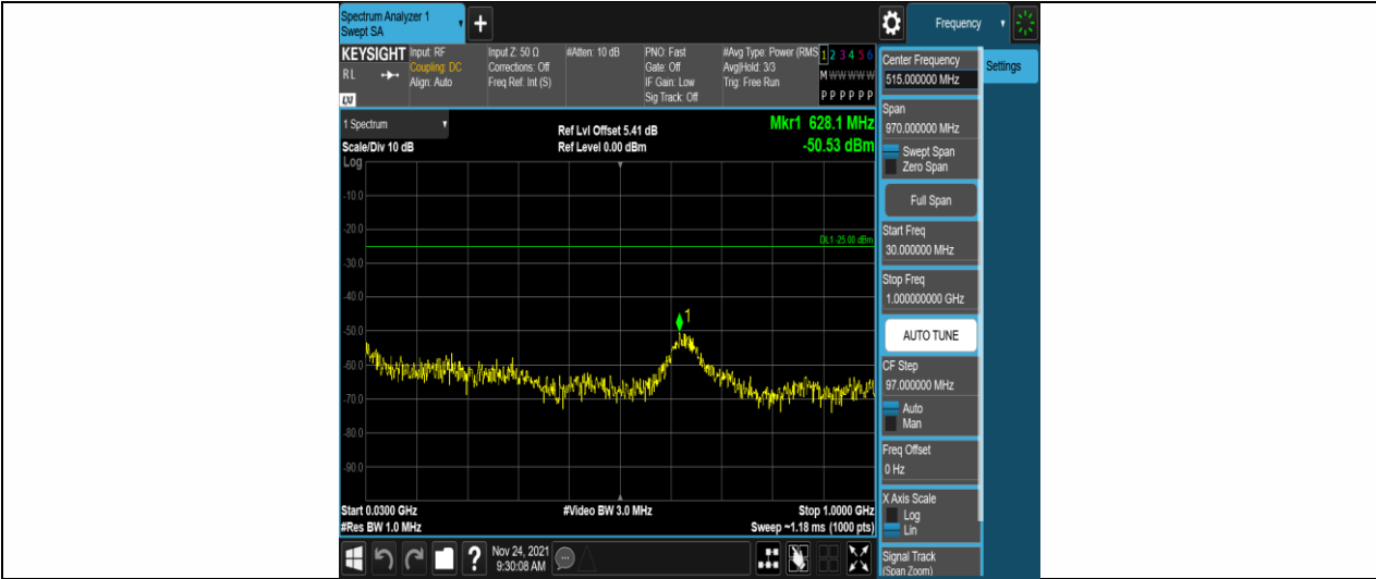
Band7-15MHz-QPSK-21375-75RB#0-Range1:30~1000MHz
