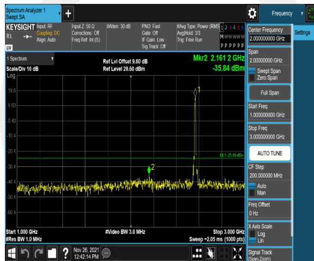
Band7-20MHz-16QAM -21350-100RB#0-Range1:1000~3000MHz
