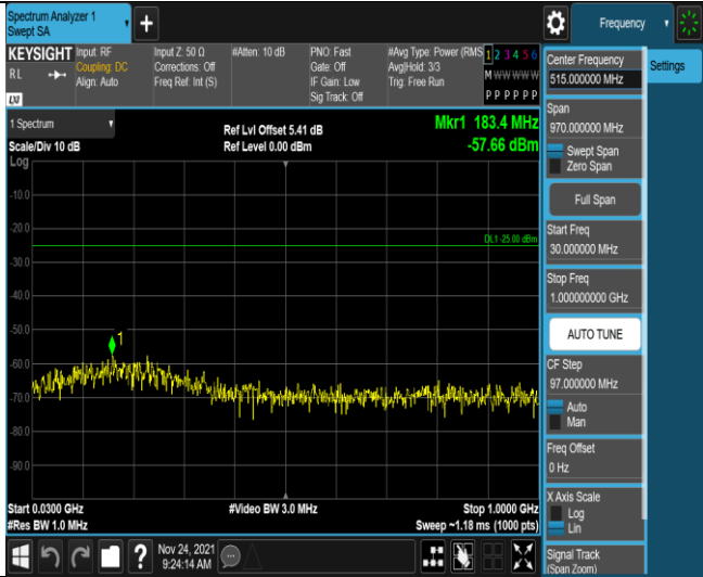
Band7-10MHz-16QAM-21400-50RB#0-Range1:30~1000MHz
