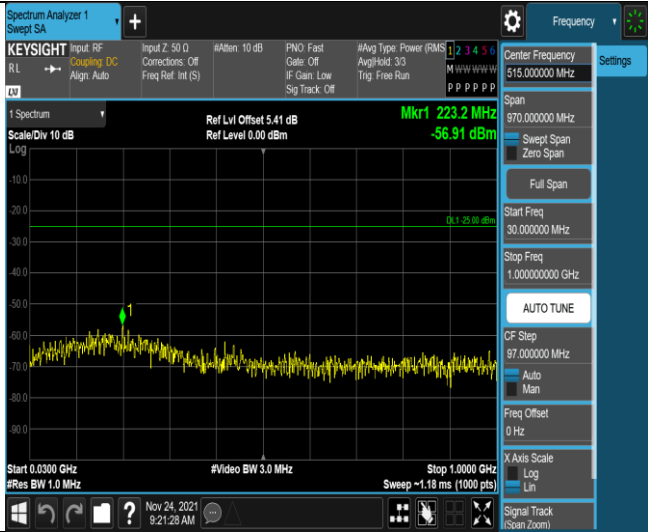
Band7-10MHz-16QAM-20800-50RB#0-Range1:30~1000MHz
