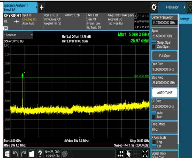
Band7-5MHz-16QAM-21100-25RB#0-Range3:3000~26500MHz
