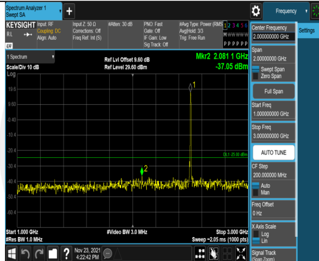
Band7-5MHz-16QAM-20775-25RB#0-Range2:1000~3000MHz
