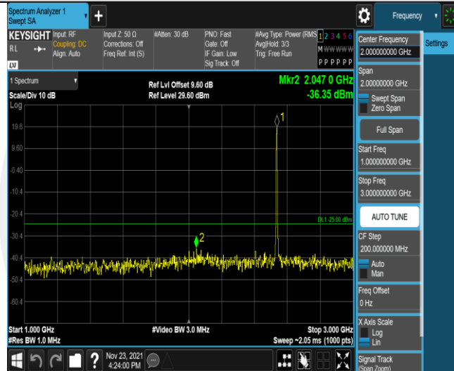
Band7-5MHz-16QAM-21100-25RB#0-Range2:1000~3000MHz
