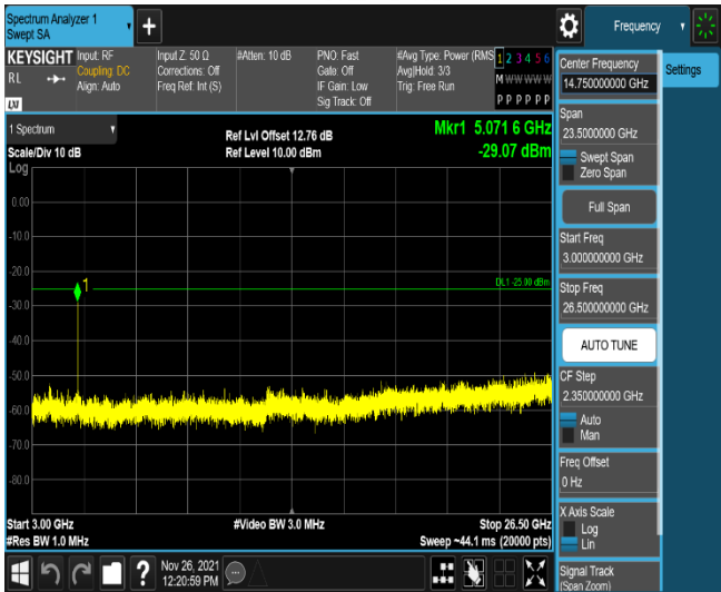
Band7-10MHz-16QAM-21400-50RB#0-Range3:3000~26500MHz
