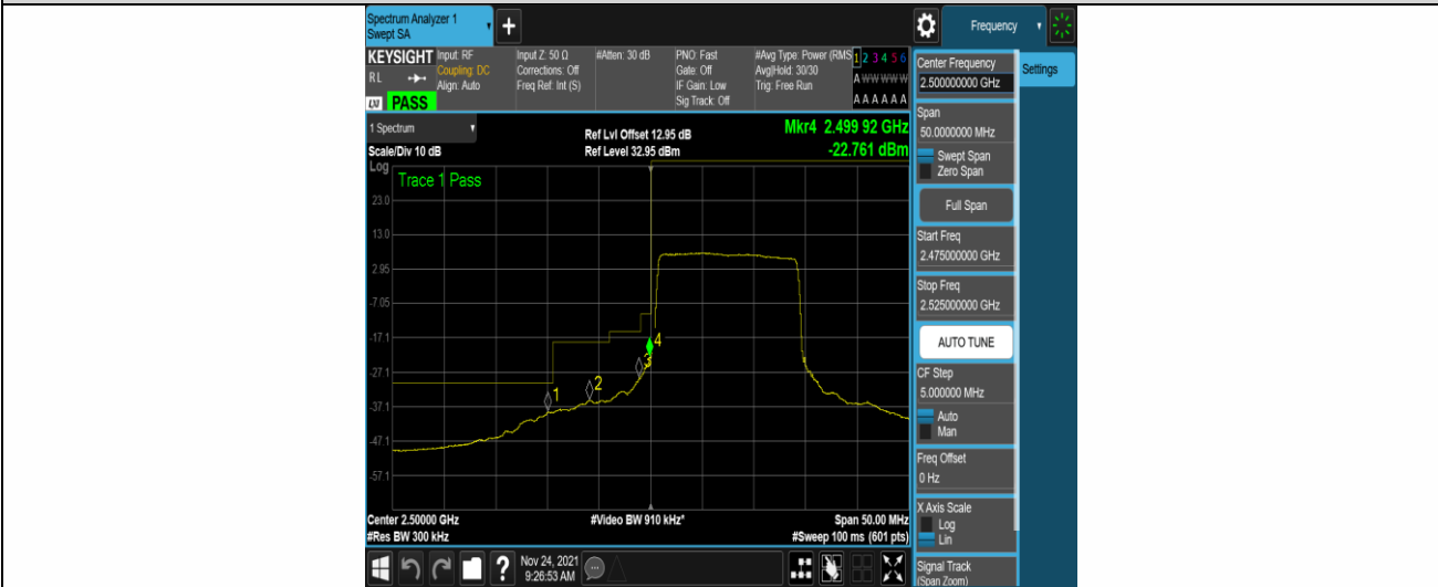
Band7-15MHz-QPSK-20825-75RB#0
