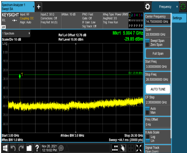
Band7-10MHz-16QAM-21100-50RB#0-Range3:3000~26500MHz
