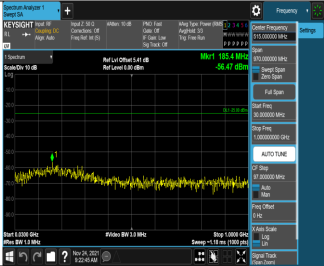
Band7-10MHz-16QAM-21100-50RB#0-Range1:30~1000MHz
