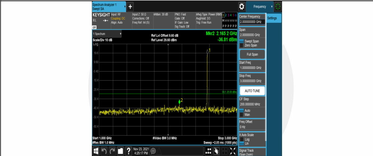
Band7-5MHz-16QAM-21425-25RB#0-Range2:1000~3000MHz
