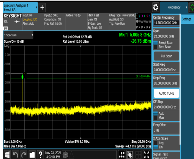
Band7-5MHz-16QAM-20775-25RB#0-Range3:3000~26500MHz
