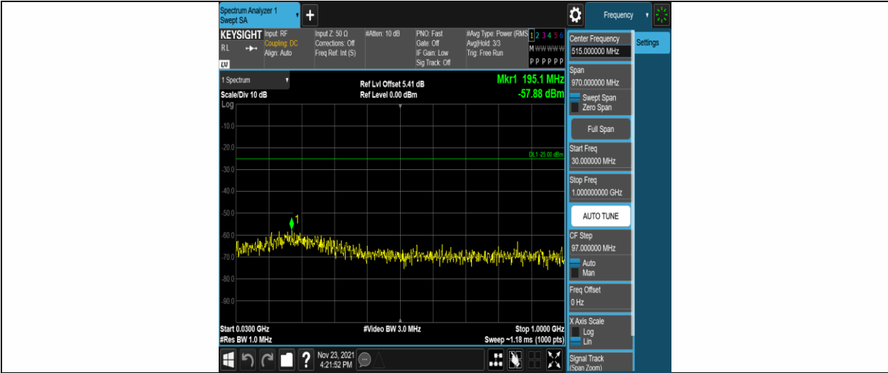
Band7-5MHz-QPSK-20775-25RB#0-Range1:30~1000MHz
