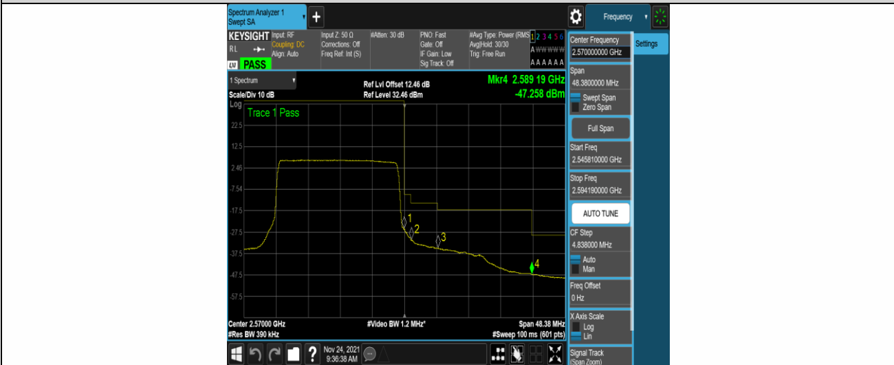
Band7-20MHz-QPSK-21350-100RB#0
