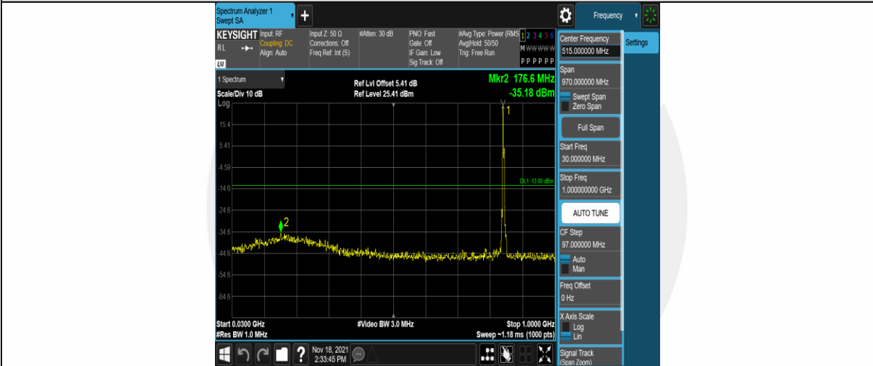
Band5-5MHz-QPSK-20625-1RB#0-Range1:30~1000MHz
