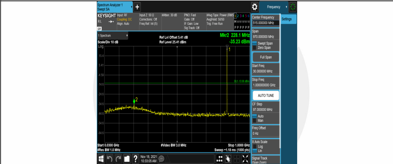
Band5-1.4MHz-16QAM-20643-1RB#0-Range1:30~1000MHz
