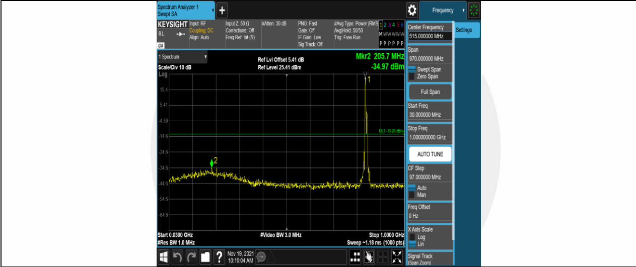
Band5-10MHz-QPSK-20600-1RB#0-Range1:30~1000MHz
