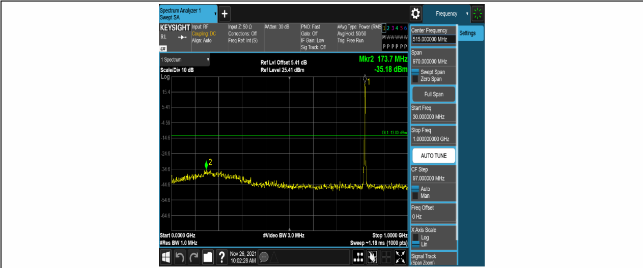
Band5-10MHz-16QAM-20450-1RB#0-Range1:30~1000MHz
