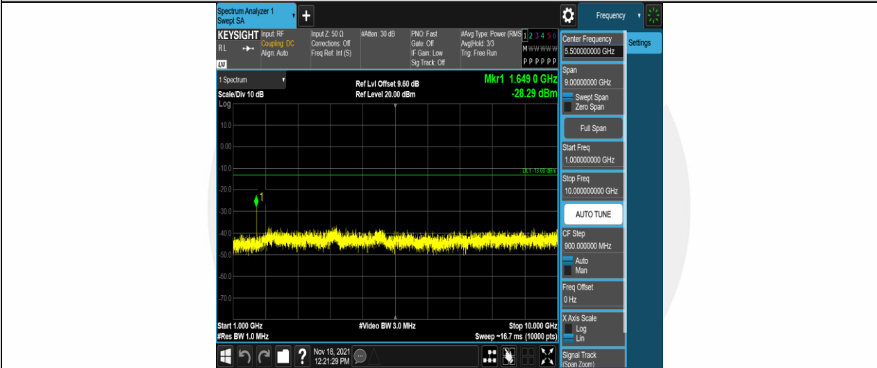
Band5-3MHz-16QAM-20415-1RB#0-Range2:1000~10000MHz
