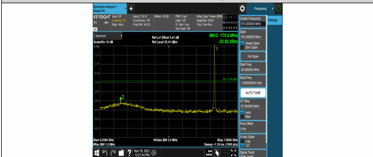
Band5-3MHz-QPSK-20525-1RB#0-Range1:30~1000MHz
