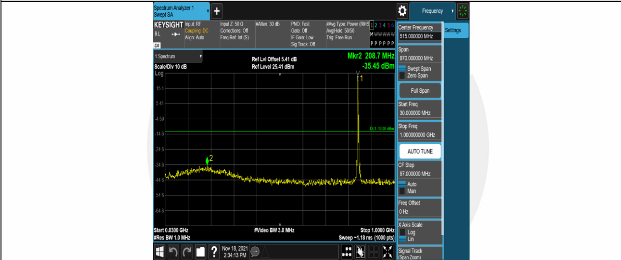
Band5-5MHz-16QAM-20625-1RB#0-Range1:30~1000MHz
