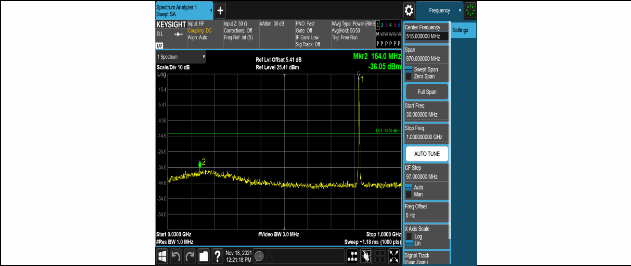
Band5-3MHz-16QAM-20415-1RB#0-Range1:30~1000MHz
