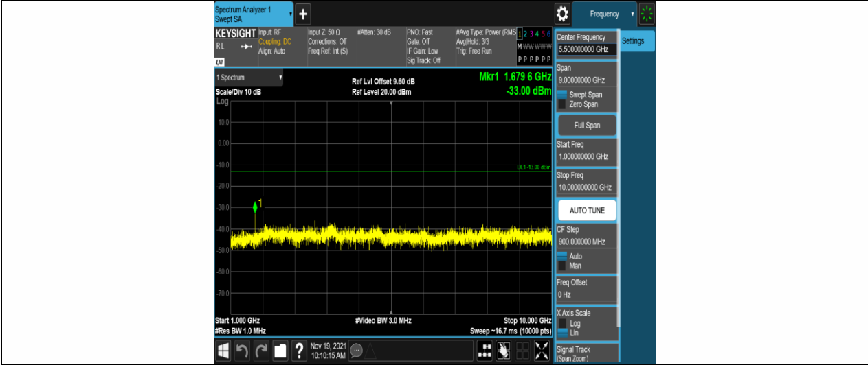
Band5-10MHz-QPSK-20600-1RB#0-Range2:1000~10000MHz
