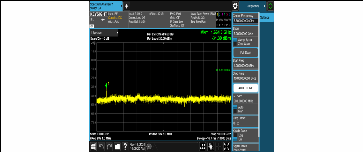
Band5-10MHz-QPSK-20525-1RB#0-Range2:1000~10000MHz
