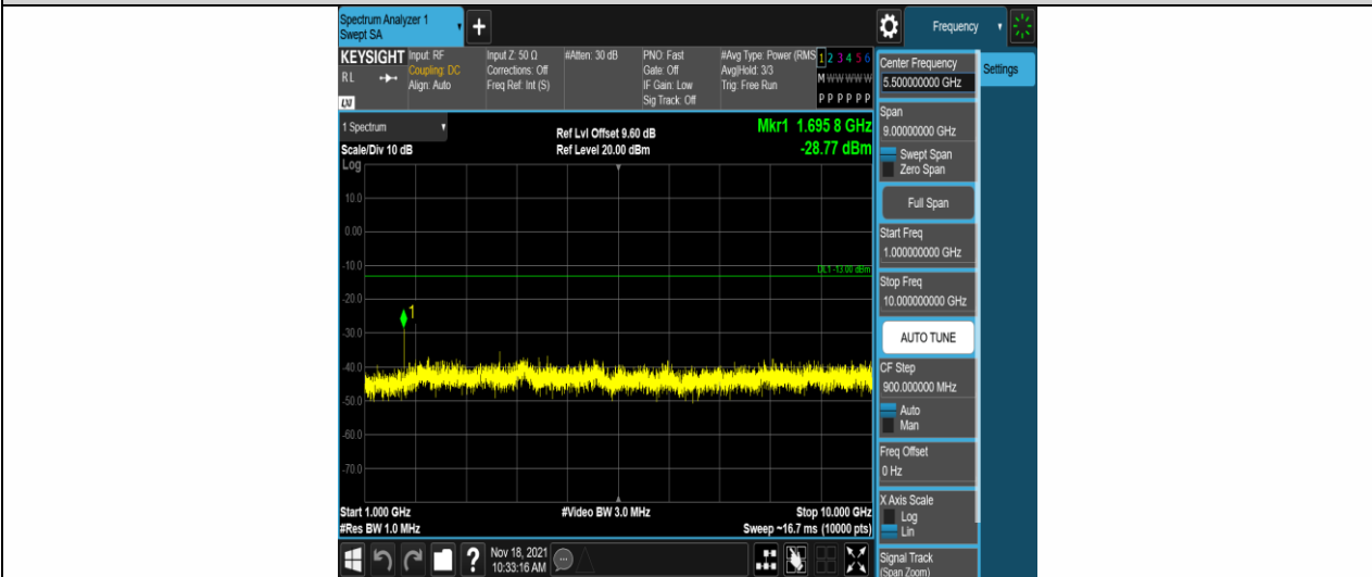
Band5-1.4MHz-16QAM-20643-1RB#0-Range2:1000~10000MHz
