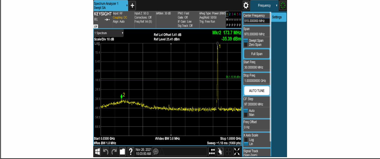
Band5-10MHz-16QAM-20525-1RB#0-Range1:30~1000MHz
