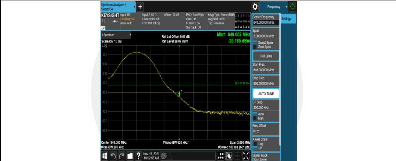
Band5-10MHz-16QAM-20600-1RB#49
