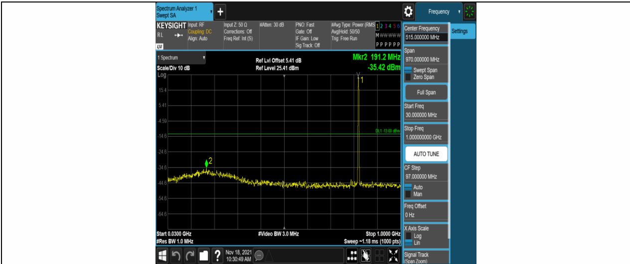
Band5-1.4MHz-QPSK-20407-1RB#0-Range1:30~1000MHz
