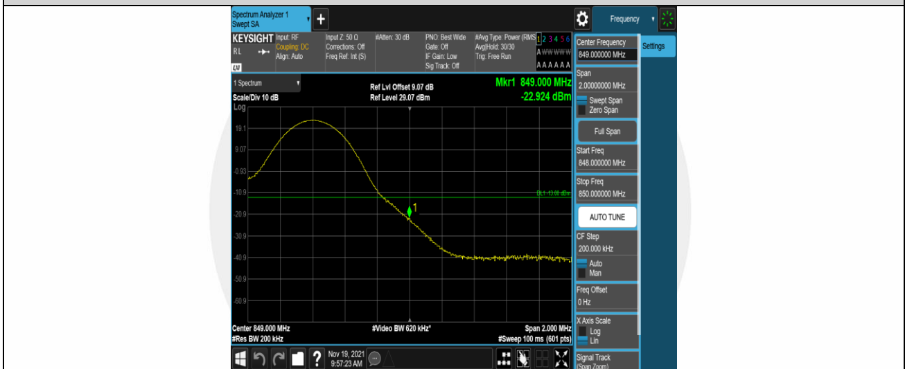
Band5-10MHz-QPSK-20600-1RB#49
