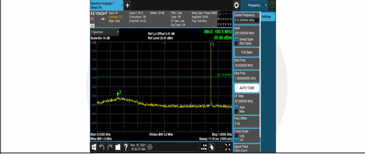
Band5-1.4MHz-QPSK-20643-1RB#0-Range1:30~1000MHz
