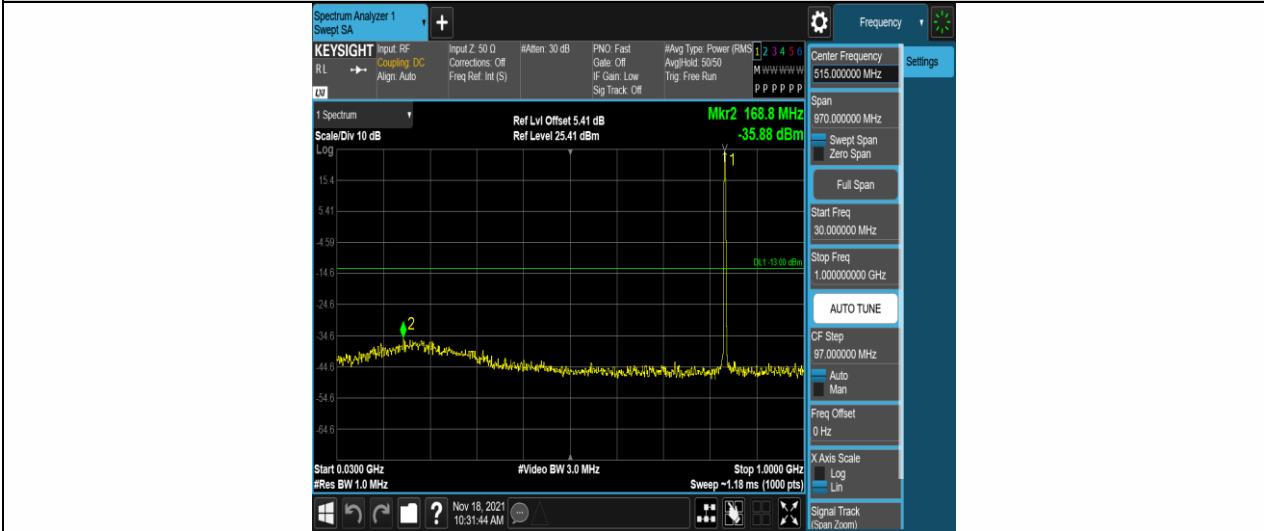
Band5-1.4MHz-QPSK-20525-1RB#0-Range1:30~1000MHz
